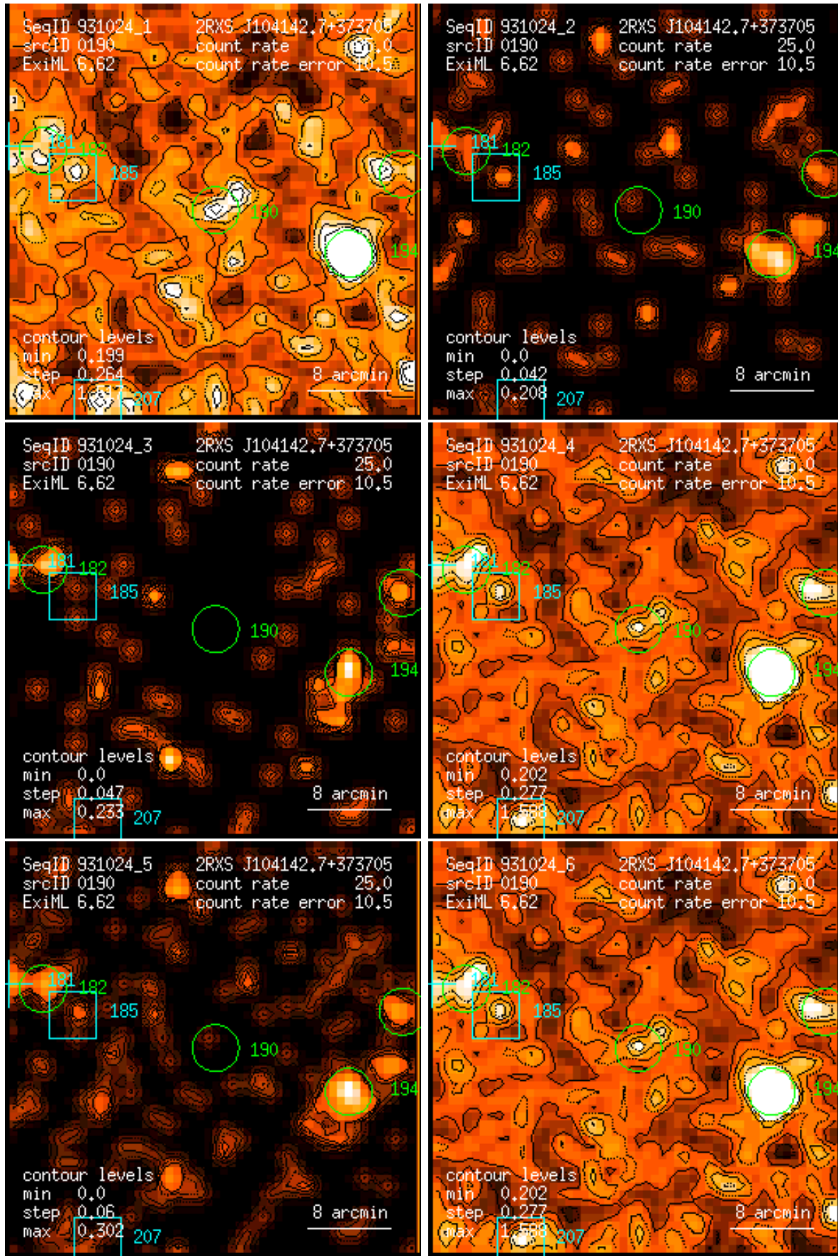
Figure 190: RASS 931024: detection 0190: band rate images, Gaussian filter: (1) PSPC channels 11 – 41, (2) 52 – 90, (3) 91 – 201, (4) 11 – 235, (5) 52 – 201, (6) 11 – 201. Broad band rates in counts/ks. Band rate contour levels in counts/ks/arcmin 2 .
