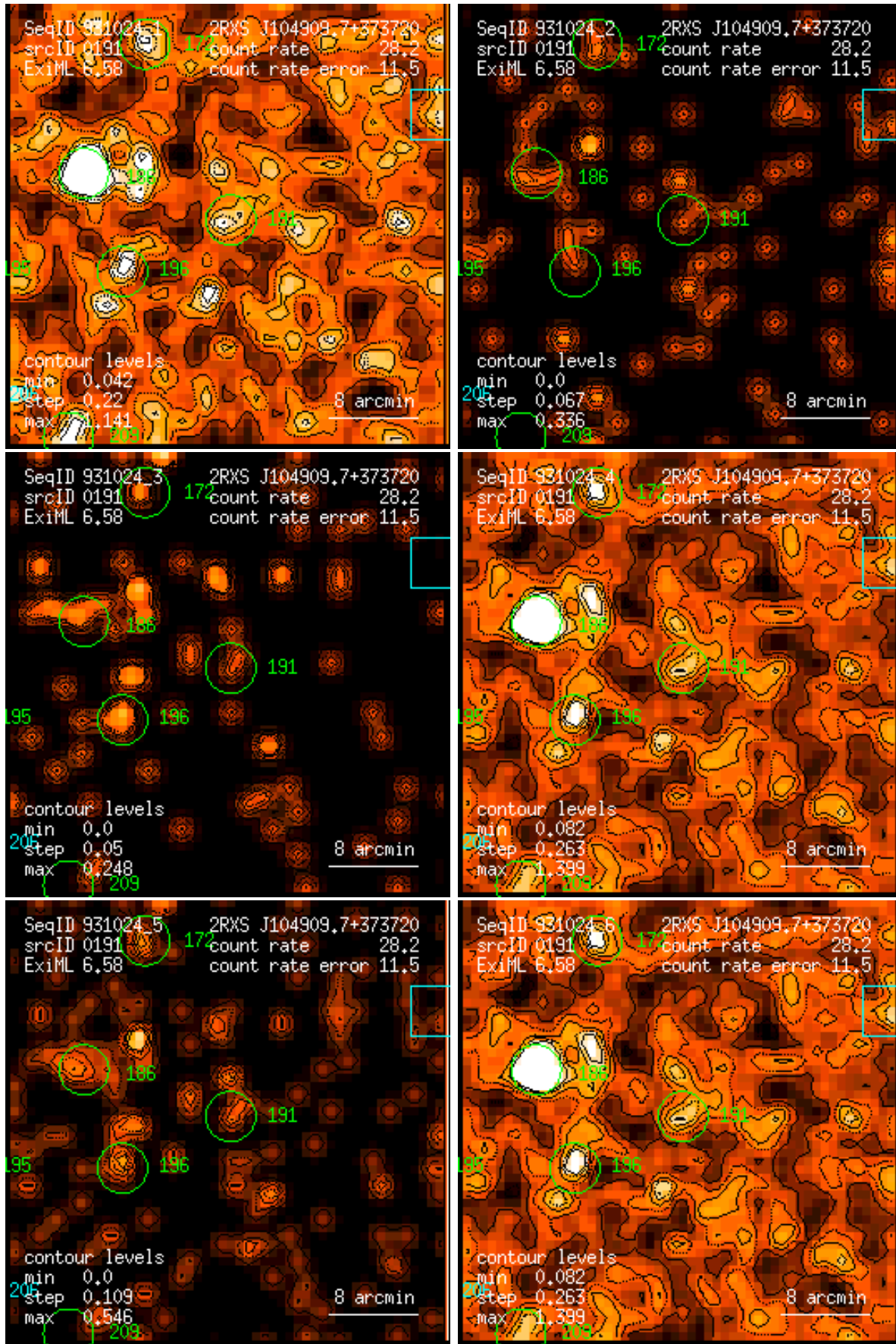
Figure 191: RASS 931024: detection 0191: band rate images, Gaussian filter: (1) PSPC channels 11 – 41, (2) 52 – 90, (3) 91 – 201, (4) 11 – 235, (5) 52 – 201, (6) 11 – 201. Broad band rates in counts/ks. Band rate contour levels in counts/ks/arcmin 2 .
