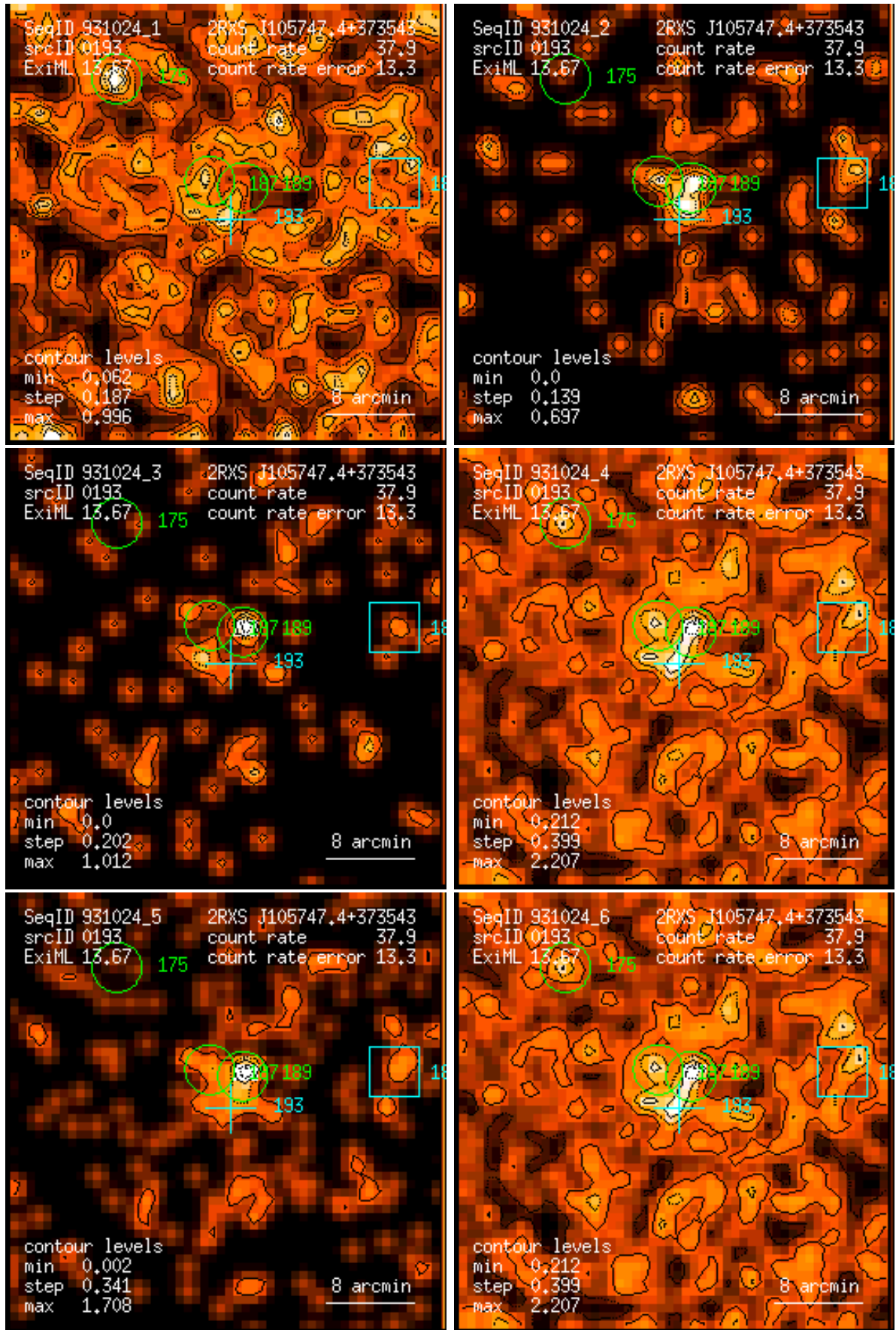
Figure 193: RASS 931024: detection 0193: band rate images, Gaussian filter: (1) PSPC channels 11 – 41, (2) 52 – 90, (3) 91 – 201, (4) 11 – 235, (5) 52 – 201, (6) 11 – 201. Broad band rates in counts/ks. Band rate contour levels in counts/ks/arcmin 2 .
