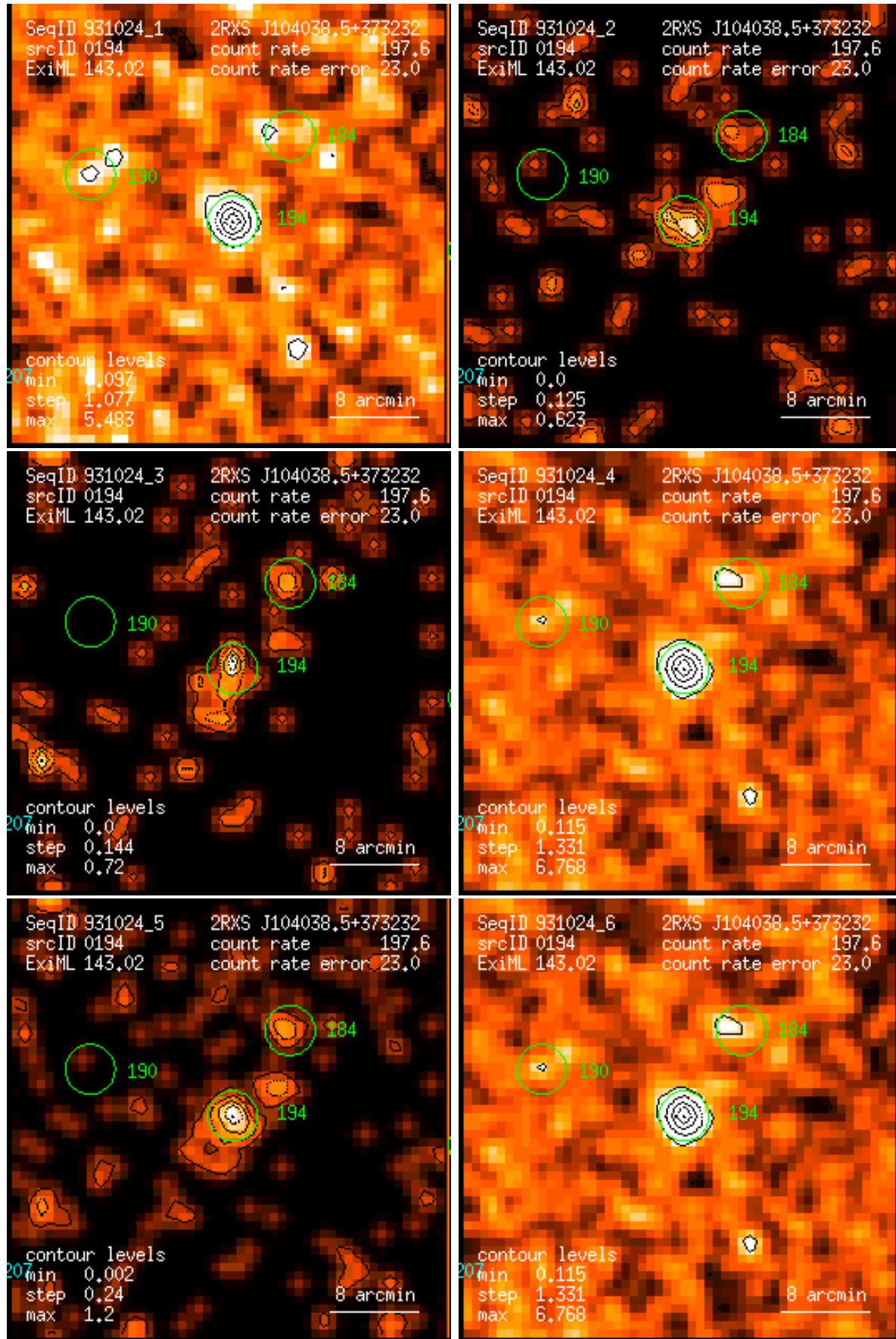
Figure 194: RASS 931024: detection 0194: band rate images, Gaussian filter: (1) PSPC channels 11 – 41, (2) 52 – 90, (3) 91 – 201, (4) 11 – 235, (5) 52 – 201, (6) 11 – 201. Broad band rates in counts/ks. Band rate contour levels in counts/ks/arcmin 2 .
