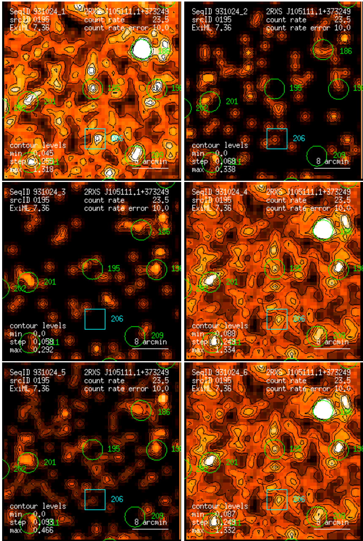
Figure 195: RASS 931024: detection 0195: band rate images, Gaussian filter: (1) PSPC channels 11 – 41, (2) 52 – 90, (3) 91 – 201, (4) 11 – 235, (5) 52 – 201, (6) 11 – 201. Broad band rates in counts/ks. Band rate contour levels in counts/ks/arcmin 2 .
