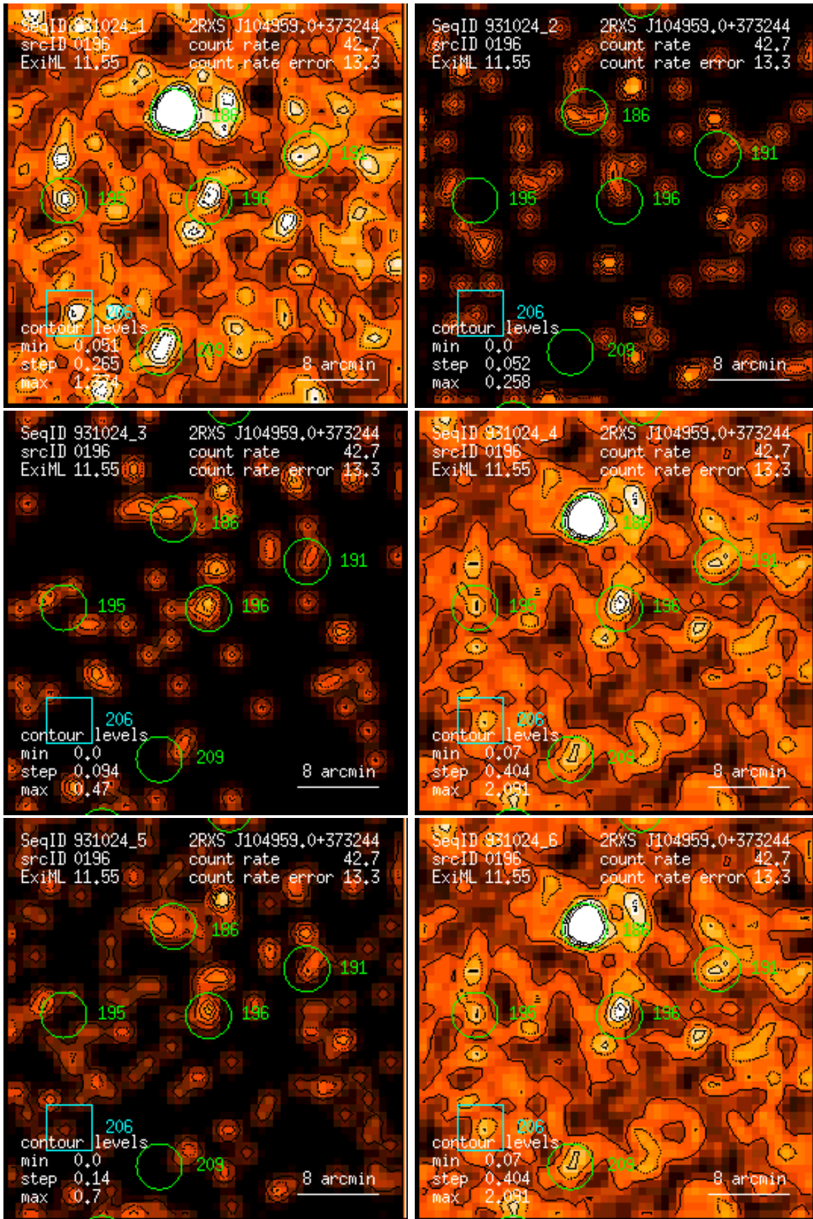
Figure 196: RASS 931024: detection 0196: band rate images, Gaussian filter: (1) PSPC channels 11 – 41, (2) 52 – 90, (3) 91 – 201, (4) 11 – 235, (5) 52 – 201, (6) 11 – 201. Broad band rates in counts/ks. Band rate contour levels in counts/ks/arcmin 2 .
