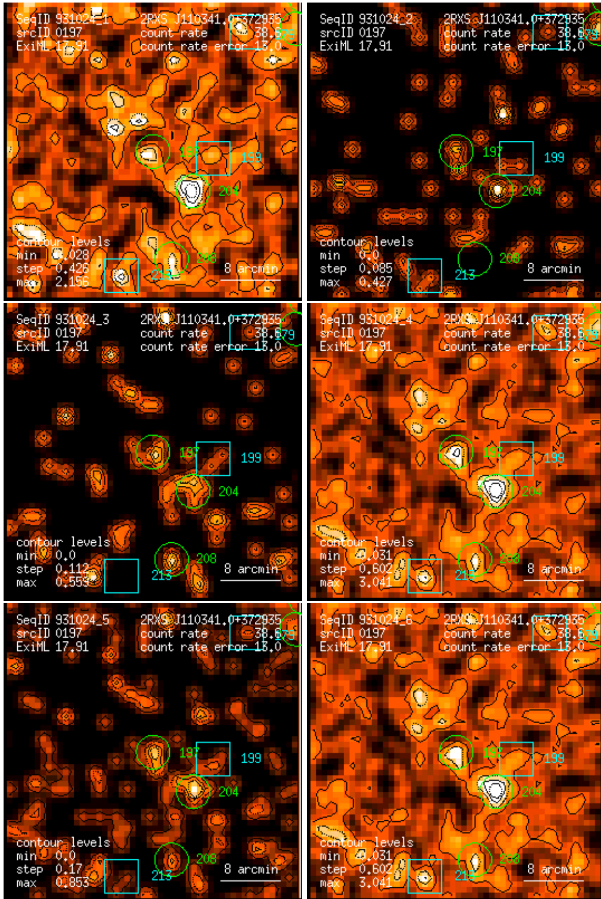
Figure 197: RASS 931024: detection 0197: band rate images, Gaussian filter: (1) PSPC channels 11 – 41, (2) 52 – 90, (3) 91 – 201, (4) 11 – 235, (5) 52 – 201, (6) 11 – 201. Broad band rates in counts/ks. Band rate contour levels in counts/ks/arcmin 2 .
