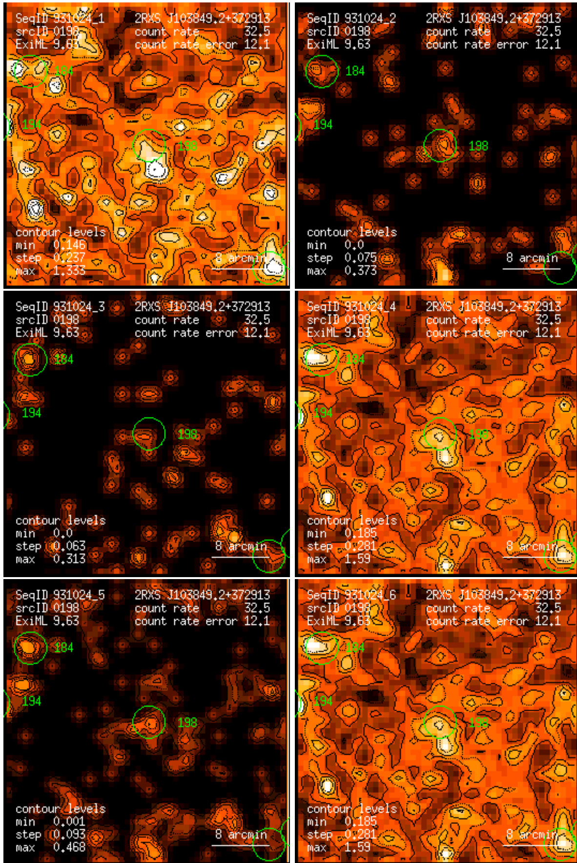
Figure 198: RASS 931024: detection 0198: band rate images, Gaussian filter: (1) PSPC channels 11 – 41, (2) 52 – 90, (3) 91 – 201, (4) 11 – 235, (5) 52 – 201, (6) 11 – 201. Broad band rates in counts/ks. Band rate contour levels in counts/ks/arcmin 2 .
