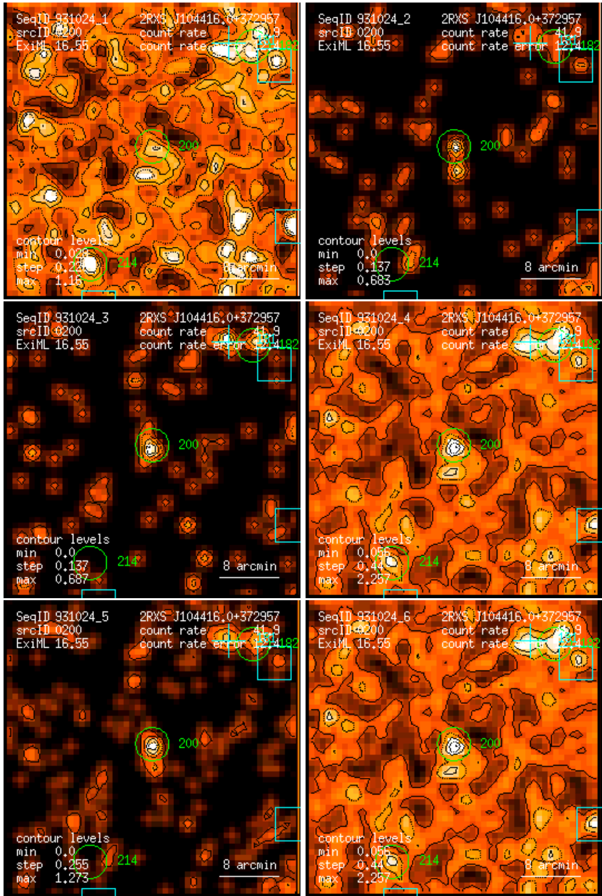
Figure 200: RASS 931024: detection 0200: band rate images, Gaussian filter: (1) PSPC channels 11 – 41, (2) 52 – 90, (3) 91 – 201, (4) 11 – 235, (5) 52 – 201, (6) 11 – 201. Broad band rates in counts/ks. Band rate contour levels in counts/ks/arcmin 2 .
