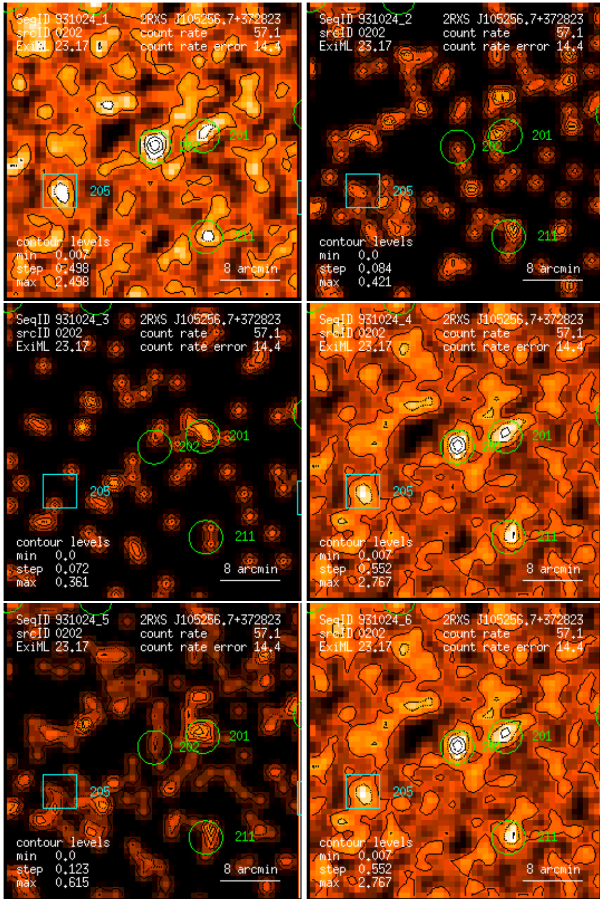
Figure 202: RASS 931024: detection 0202: band rate images, Gaussian filter: (1) PSPC channels 11 – 41, (2) 52 – 90, (3) 91 – 201, (4) 11 – 235, (5) 52 – 201, (6) 11 – 201. Broad band rates in counts/ks. Band rate contour levels in counts/ks/arcmin 2 .
