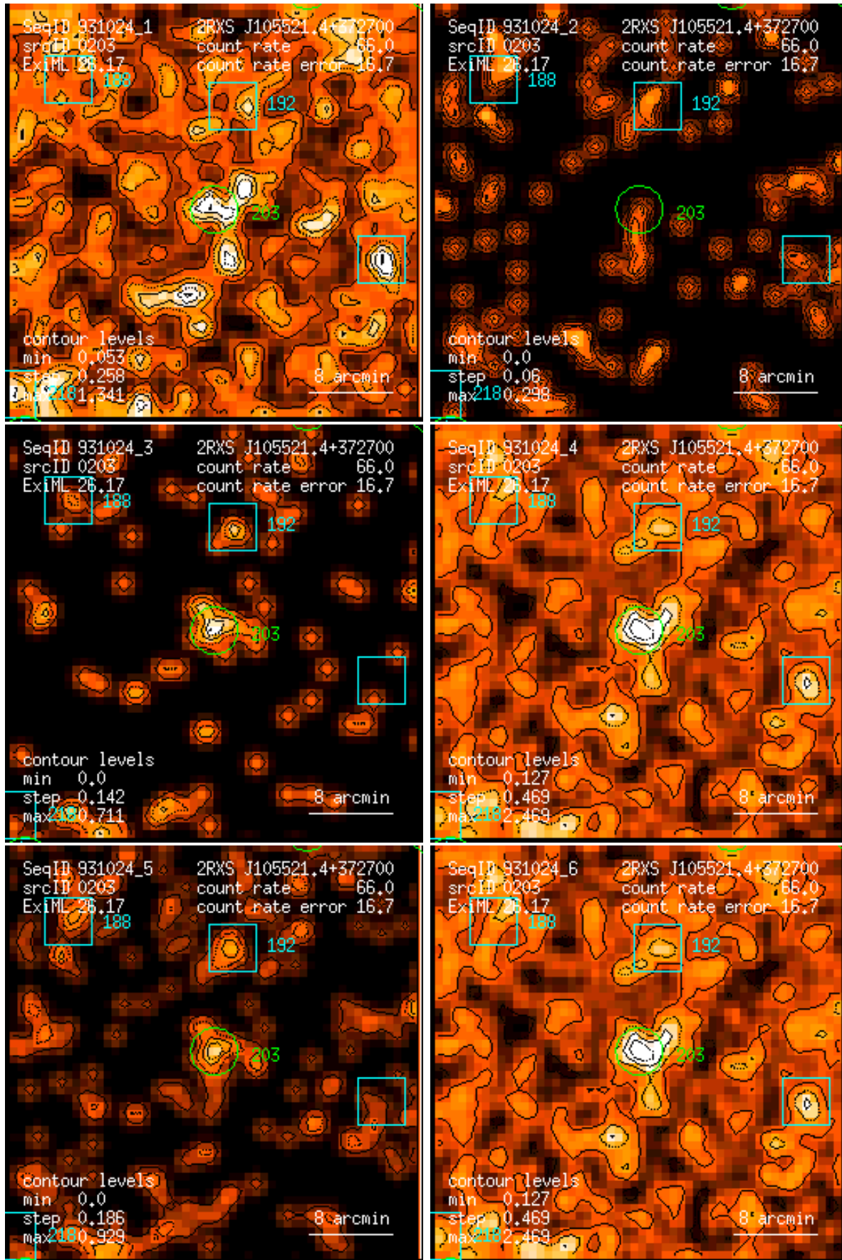
Figure 203: RASS 931024: detection 0203: band rate images, Gaussian filter: (1) PSPC channels 11 – 41, (2) 52 – 90, (3) 91 – 201, (4) 11 – 235, (5) 52 – 201, (6) 11 – 201. Broad band rates in counts/ks. Band rate contour levels in counts/ks/arcmin 2 .
