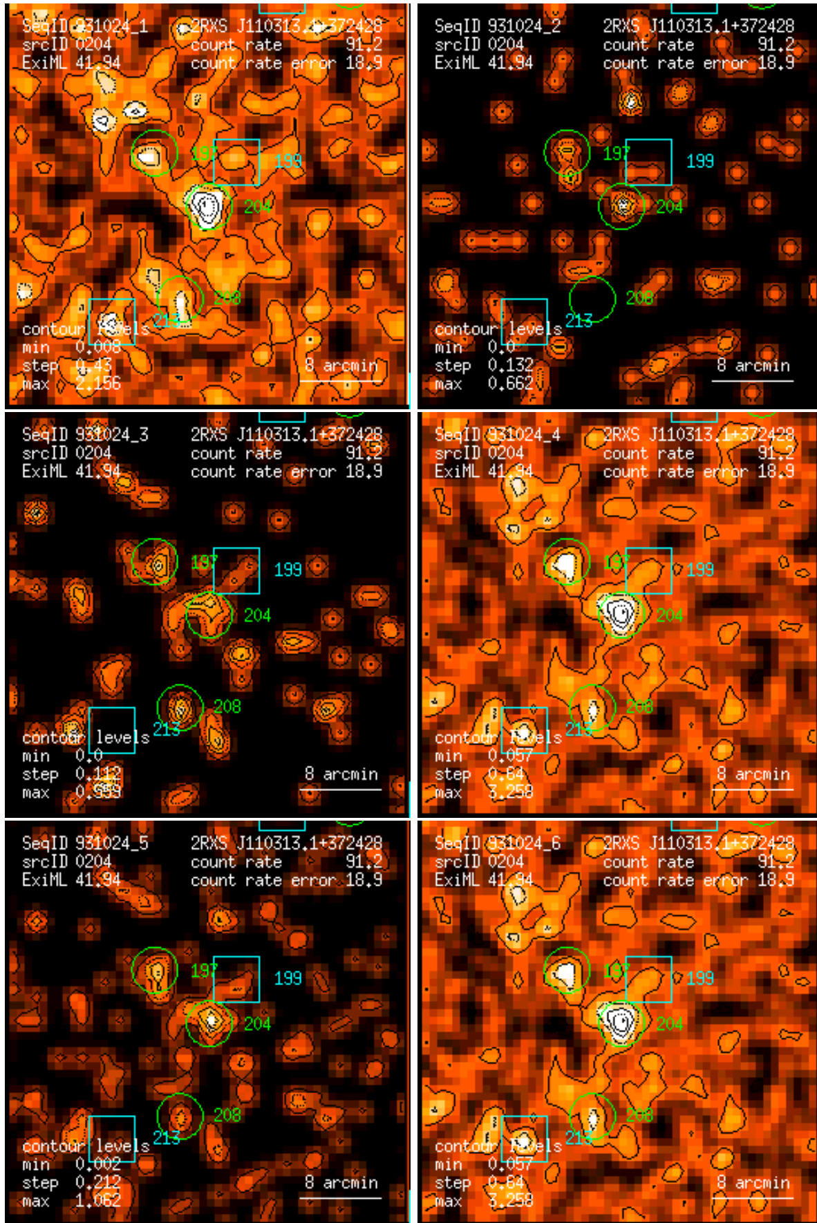
Figure 204: RASS 931024: detection 0204: band rate images, Gaussian filter: (1) PSPC channels 11 – 41, (2) 52 – 90, (3) 91 – 201, (4) 11 – 235, (5) 52 – 201, (6) 11 – 201. Broad band rates in counts/ks. Band rate contour levels in counts/ks/arcmin 2 .
