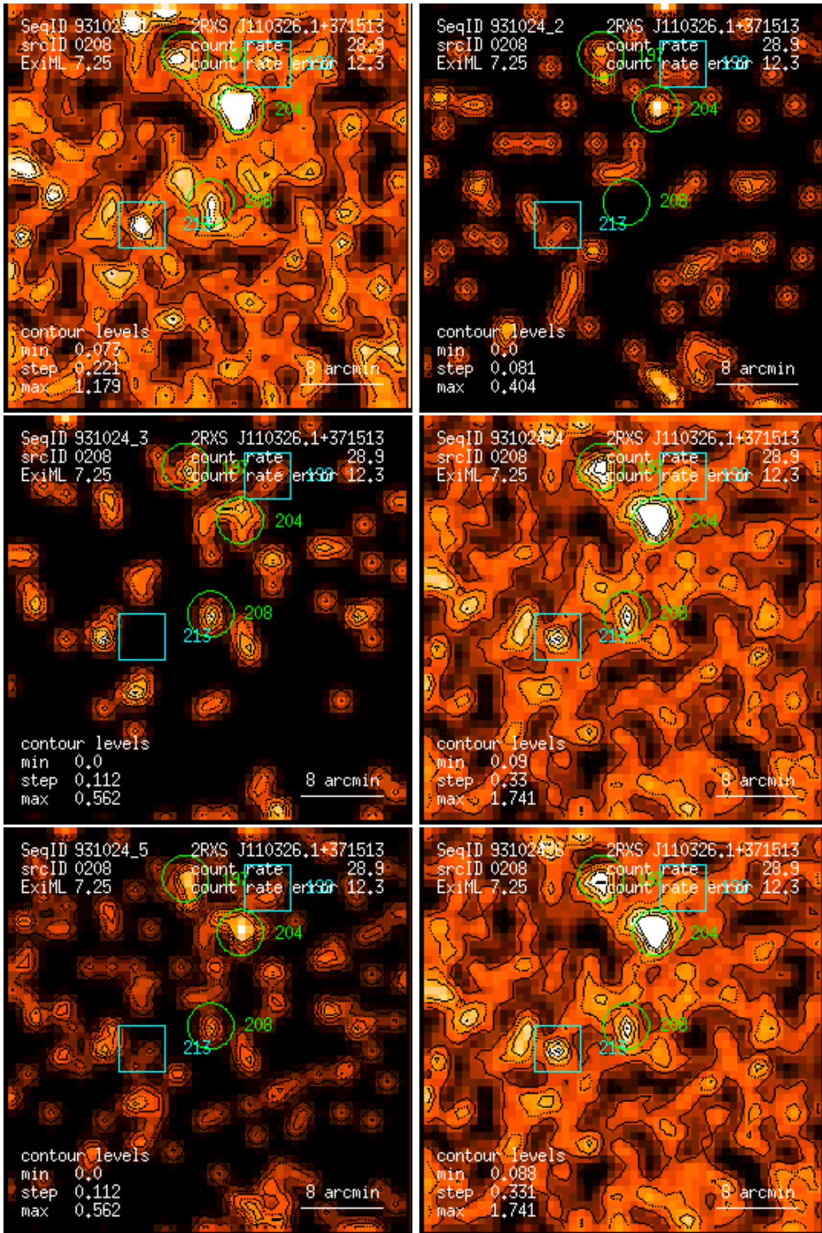
Figure 208: RASS 931024: detection 0208: band rate images, Gaussian filter: (1) PSPC channels 11 – 41, (2) 52 – 90, (3) 91 – 201, (4) 11 – 235, (5) 52 – 201, (6) 11 – 201. Broad band rates in counts/ks. Band rate contour levels in counts/ks/arcmin 2 .
