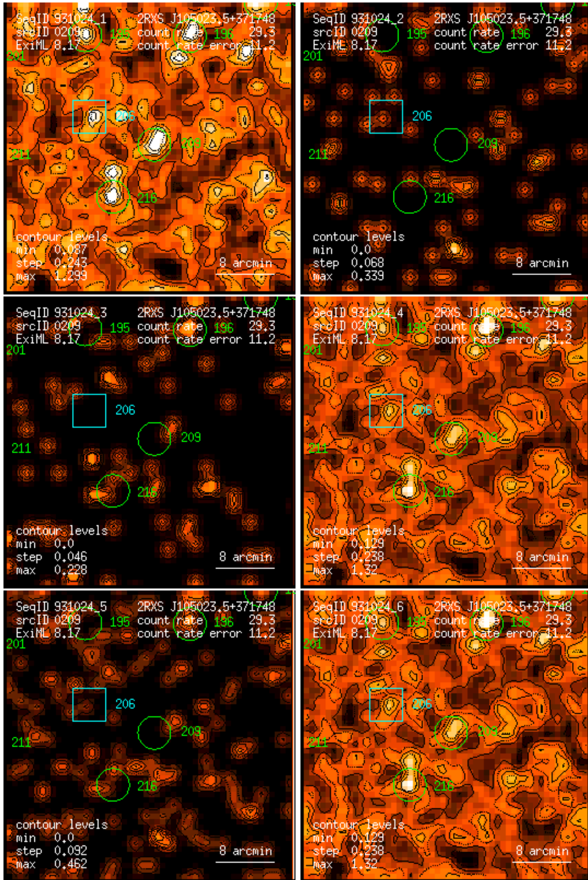
Figure 209: RASS 931024: detection 0209: band rate images, Gaussian filter: (1) PSPC channels 11 – 41, (2) 52 – 90, (3) 91 – 201, (4) 11 – 235, (5) 52 – 201, (6) 11 – 201. Broad band rates in counts/ks. Band rate contour levels in counts/ks/arcmin 2 .
