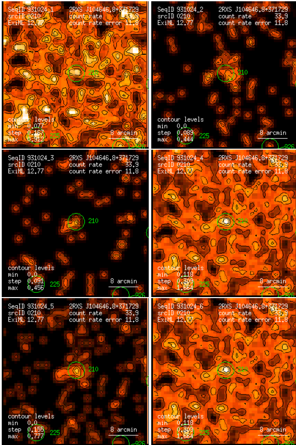
Figure 210: RASS 931024: detection 0210: band rate images, Gaussian filter: (1) PSPC channels 11 – 41, (2) 52 – 90, (3) 91 – 201, (4) 11 – 235, (5) 52 – 201, (6) 11 – 201. Broad band rates in counts/ks. Band rate contour levels in counts/ks/arcmin 2 .
