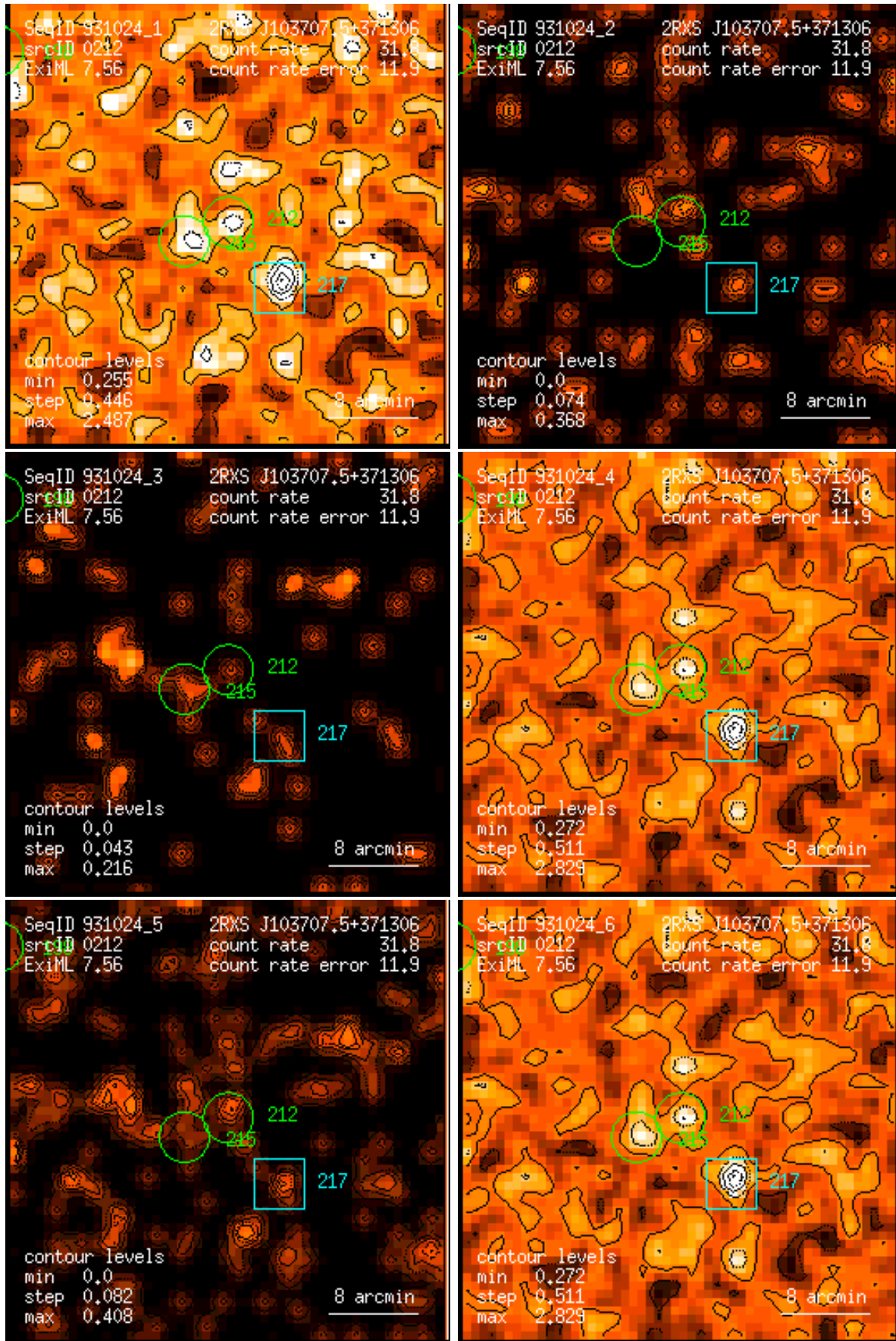
Figure 212: RASS 931024: detection 0212: band rate images, Gaussian filter: (1) PSPC channels 11 – 41, (2) 52 – 90, (3) 91 – 201, (4) 11 – 235, (5) 52 – 201, (6) 11 – 201. Broad band rates in counts/ks. Band rate contour levels in counts/ks/arcmin 2 .
