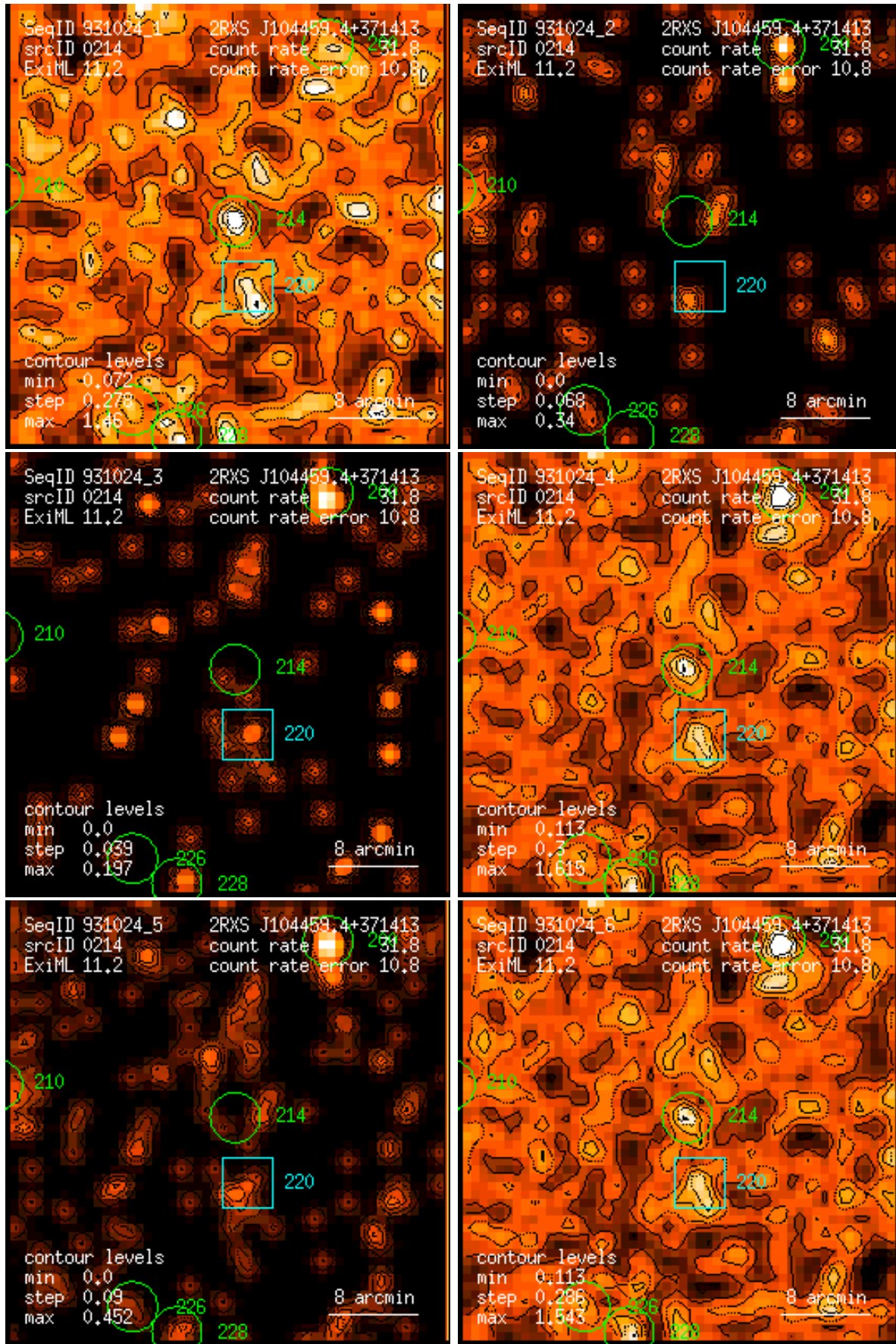
Figure 214: RASS 931024: detection 0214: band rate images, Gaussian filter: (1) PSPC channels 11 – 41, (2) 52 – 90, (3) 91 – 201, (4) 11 – 235, (5) 52 – 201, (6) 11 – 201. Broad band rates in counts/ks. Band rate contour levels in counts/ks/arcmin 2 .
