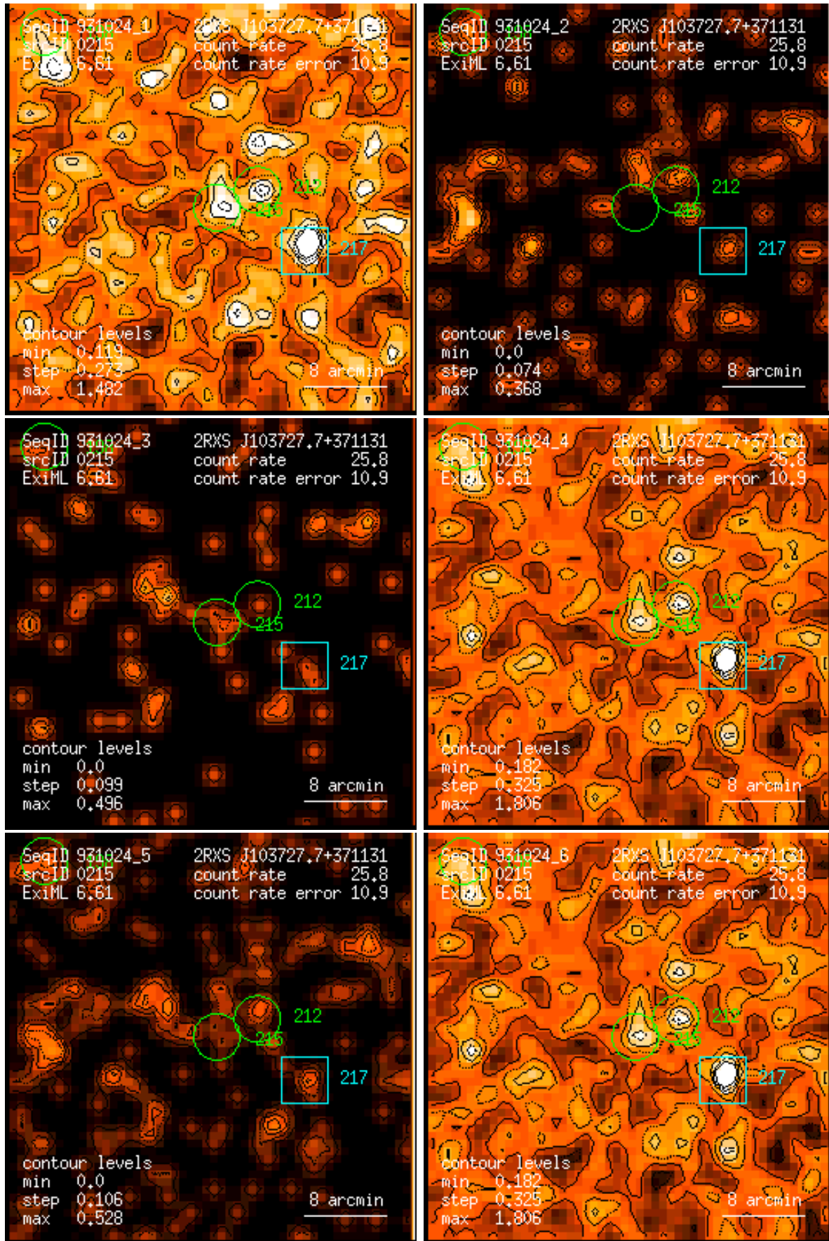
Figure 215: RASS 931024: detection 0215: band rate images, Gaussian filter: (1) PSPC channels 11 – 41, (2) 52 – 90, (3) 91 – 201, (4) 11 – 235, (5) 52 – 201, (6) 11 – 201. Broad band rates in counts/ks. Band rate contour levels in counts/ks/arcmin 2 .
