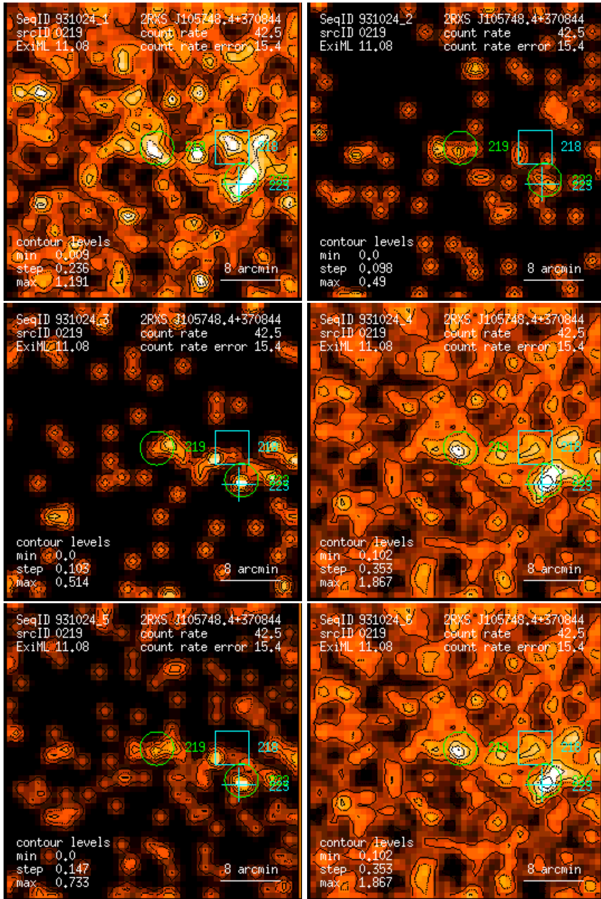
Figure 219: RASS 931024: detection 0219: band rate images, Gaussian filter: (1) PSPC channels 11 – 41, (2) 52 – 90, (3) 91 – 201, (4) 11 – 235, (5) 52 – 201, (6) 11 – 201. Broad band rates in counts/ks. Band rate contour levels in counts/ks/arcmin 2 .
