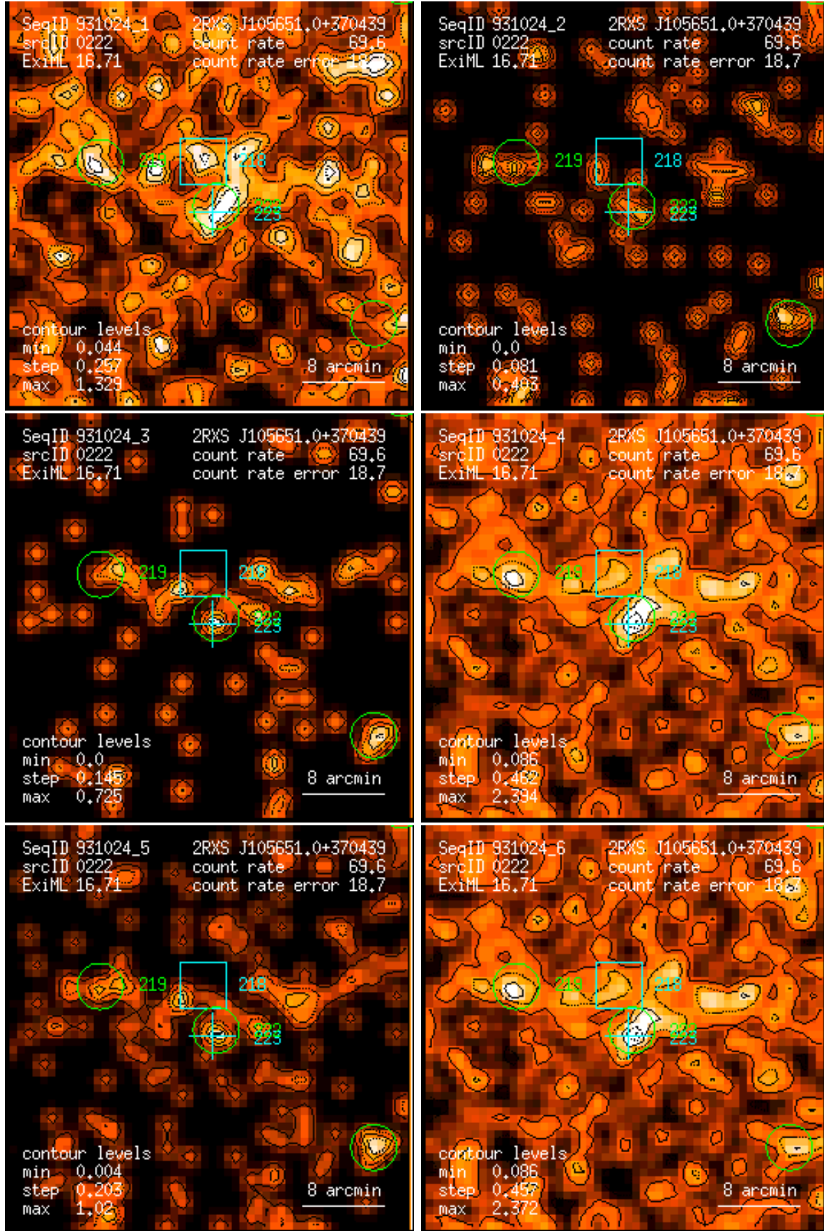
Figure 222: RASS 931024: detection 0222: band rate images, Gaussian filter: (1) PSPC channels 11 – 41, (2) 52 – 90, (3) 91 – 201, (4) 11 – 235, (5) 52 – 201, (6) 11 – 201. Broad band rates in counts/ks. Band rate contour levels in counts/ks/arcmin 2 .
