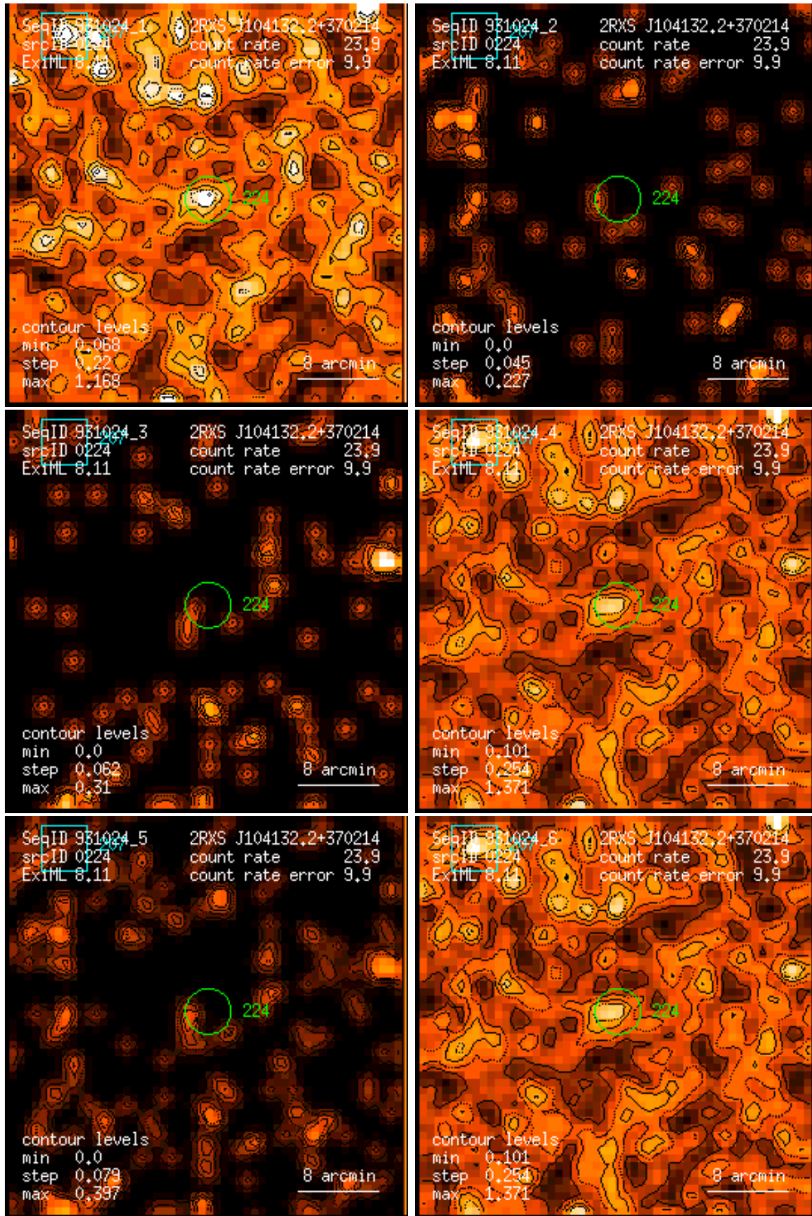
Figure 224: RASS 931024: detection 0224: band rate images, Gaussian filter: (1) PSPC channels 11 – 41, (2) 52 – 90, (3) 91 – 201, (4) 11 – 235, (5) 52 – 201, (6) 11 – 201. Broad band rates in counts/ks. Band rate contour levels in counts/ks/arcmin 2 .
