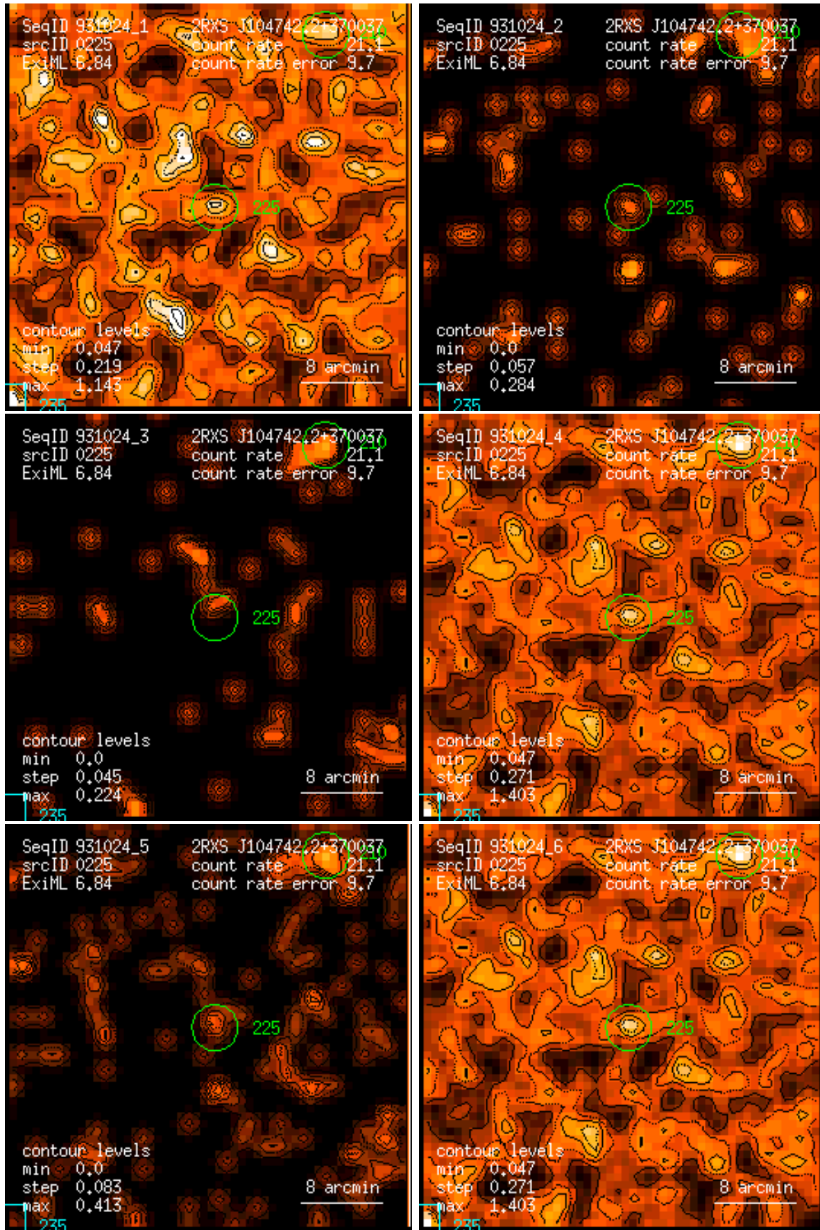
Figure 225: RASS 931024: detection 0225: band rate images, Gaussian filter: (1) PSPC channels 11 – 41, (2) 52 – 90, (3) 91 – 201, (4) 11 – 235, (5) 52 – 201, (6) 11 – 201. Broad band rates in counts/ks. Band rate contour levels in counts/ks/arcmin 2 .
