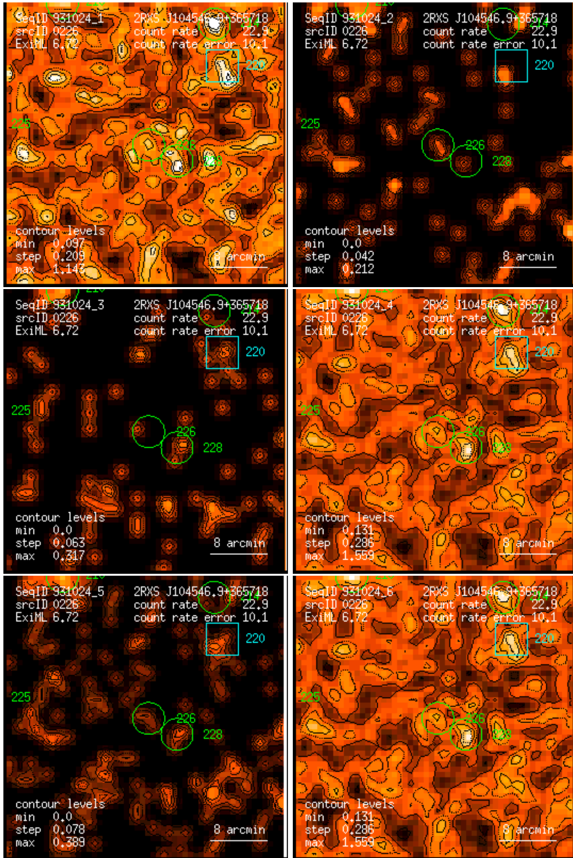
Figure 226: RASS 931024: detection 0226: band rate images, Gaussian filter: (1) PSPC channels 11 – 41, (2) 52 – 90, (3) 91 – 201, (4) 11 – 235, (5) 52 – 201, (6) 11 – 201. Broad band rates in counts/ks. Band rate contour levels in counts/ks/arcmin 2 .
