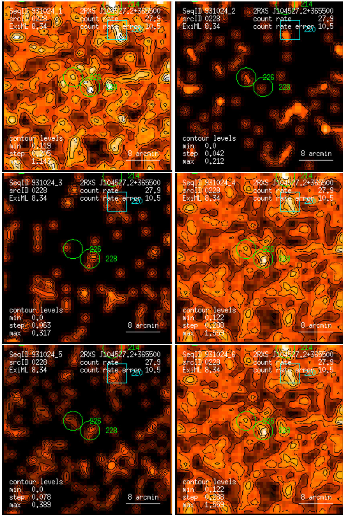
Figure 228: RASS 931024: detection 0228: band rate images, Gaussian filter: (1) PSPC channels 11 – 41, (2) 52 – 90, (3) 91 – 201, (4) 11 – 235, (5) 52 – 201, (6) 11 – 201. Broad band rates in counts/ks. Band rate contour levels in counts/ks/arcmin 2 .
