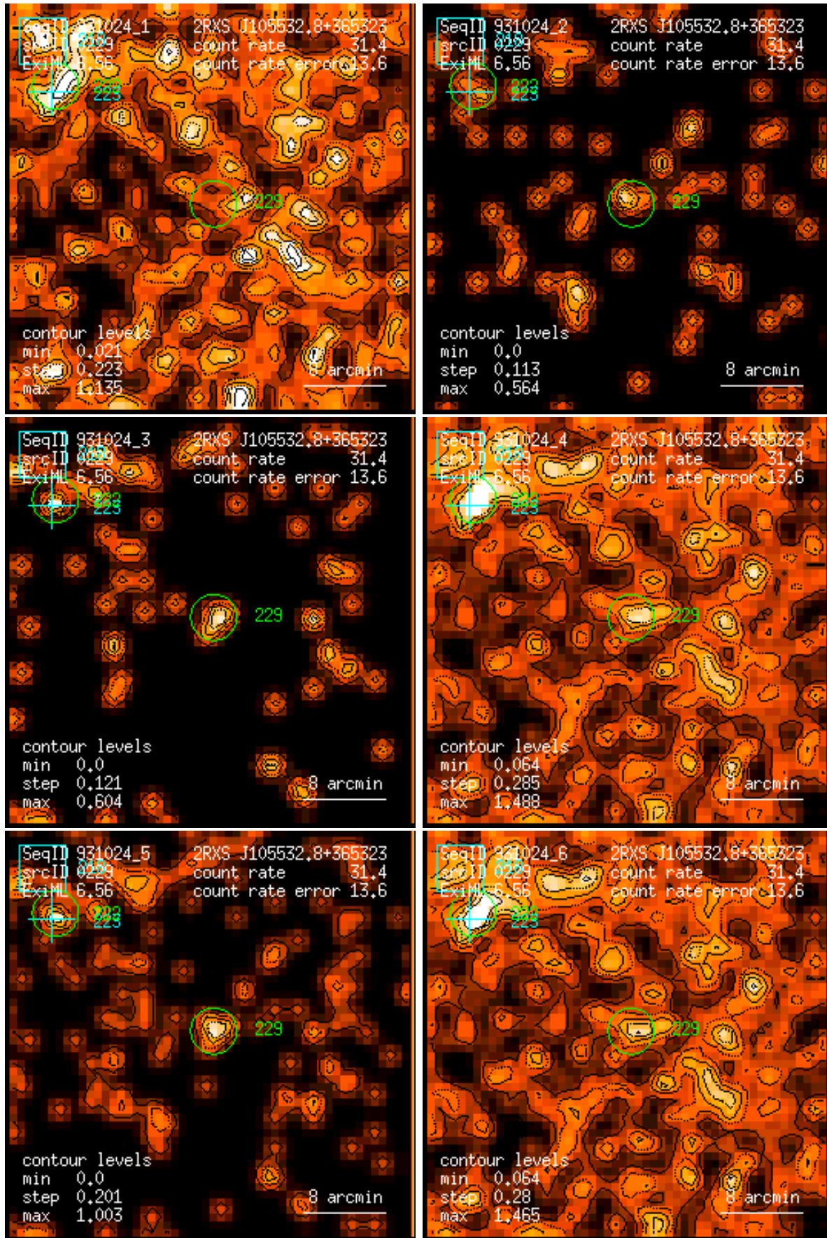
Figure 229: RASS 931024: detection 0229: band rate images, Gaussian filter: (1) PSPC channels 11 – 41, (2) 52 – 90, (3) 91 – 201, (4) 11 – 235, (5) 52 – 201, (6) 11 – 201. Broad band rates in counts/ks. Band rate contour levels in counts/ks/arcmin 2 .
