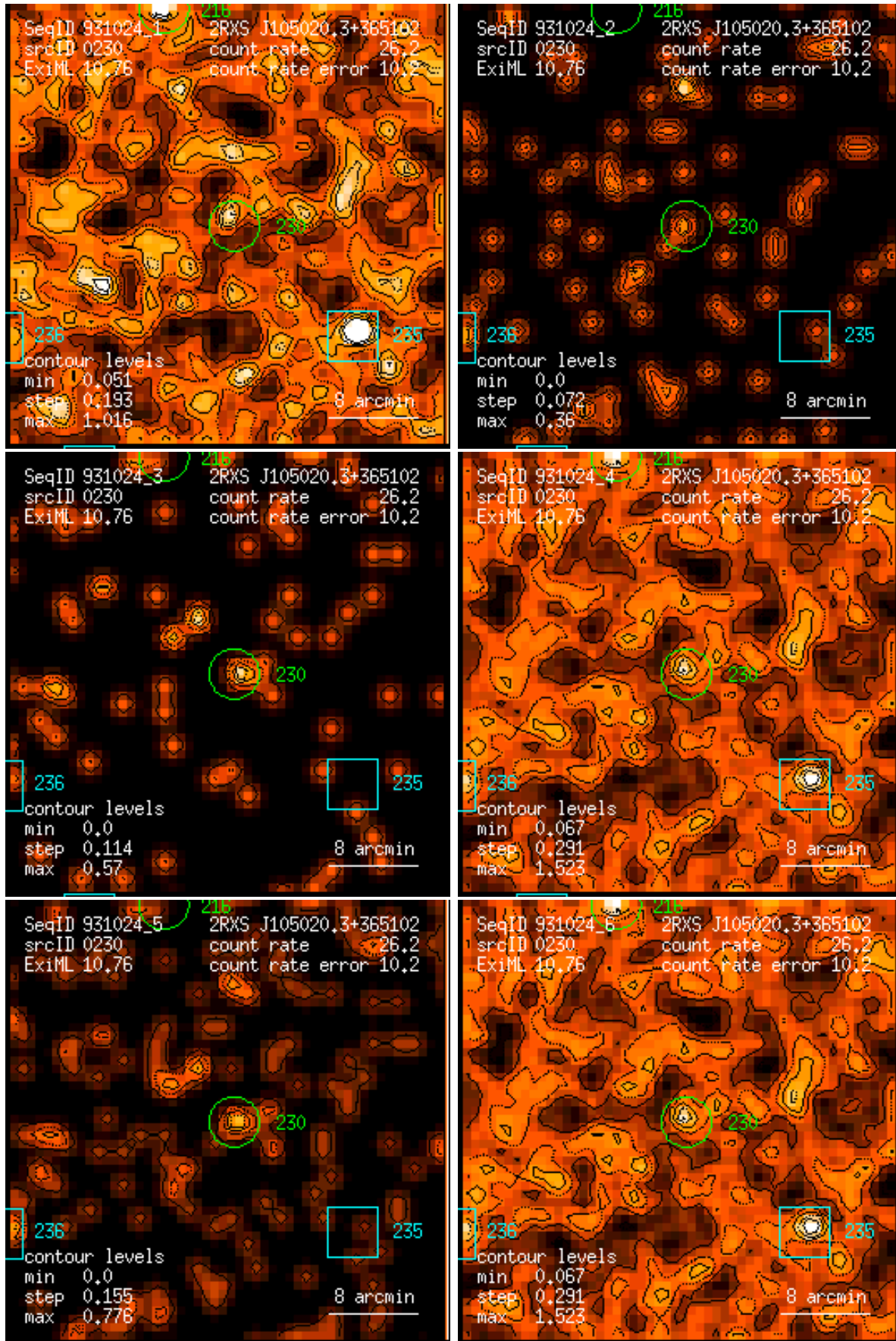
Figure 230: RASS 931024: detection 0230: band rate images, Gaussian filter: (1) PSPC channels 11 – 41, (2) 52 – 90, (3) 91 – 201, (4) 11 – 235, (5) 52 – 201, (6) 11 – 201. Broad band rates in counts/ks. Band rate contour levels in counts/ks/arcmin 2 .
