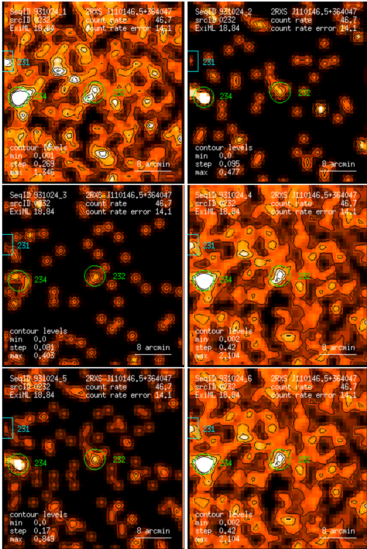
Figure 232: RASS 931024: detection 0232: band rate images, Gaussian filter: (1) PSPC channels 11 – 41, (2) 52 – 90, (3) 91 – 201, (4) 11 – 235, (5) 52 – 201, (6) 11 – 201. Broad band rates in counts/ks. Band rate contour levels in counts/ks/arcmin 2 .
