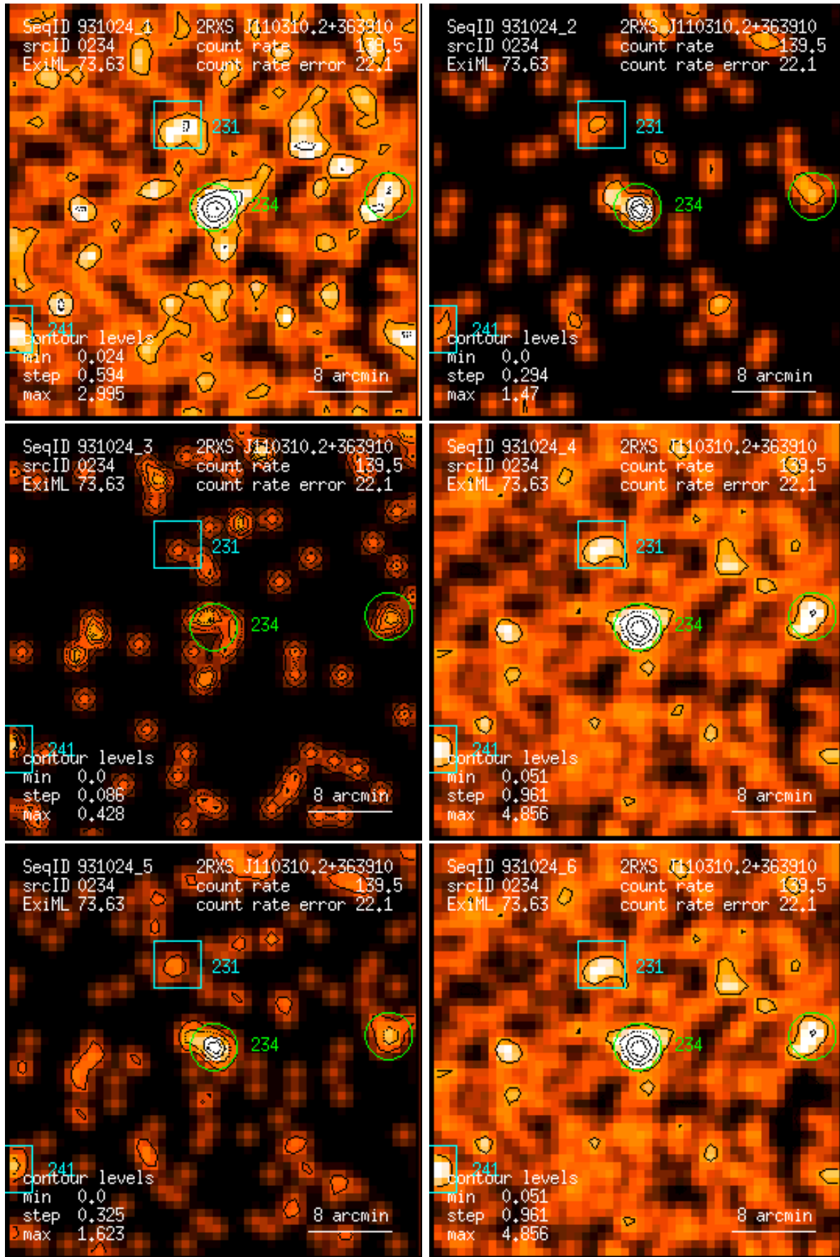
Figure 234: RASS 931024: detection 0234: band rate images, Gaussian filter: (1) PSPC channels 11 – 41, (2) 52 – 90, (3) 91 – 201, (4) 11 – 235, (5) 52 – 201, (6) 11 – 201. Broad band rates in counts/ks. Band rate contour levels in counts/ks/arcmin 2 .
