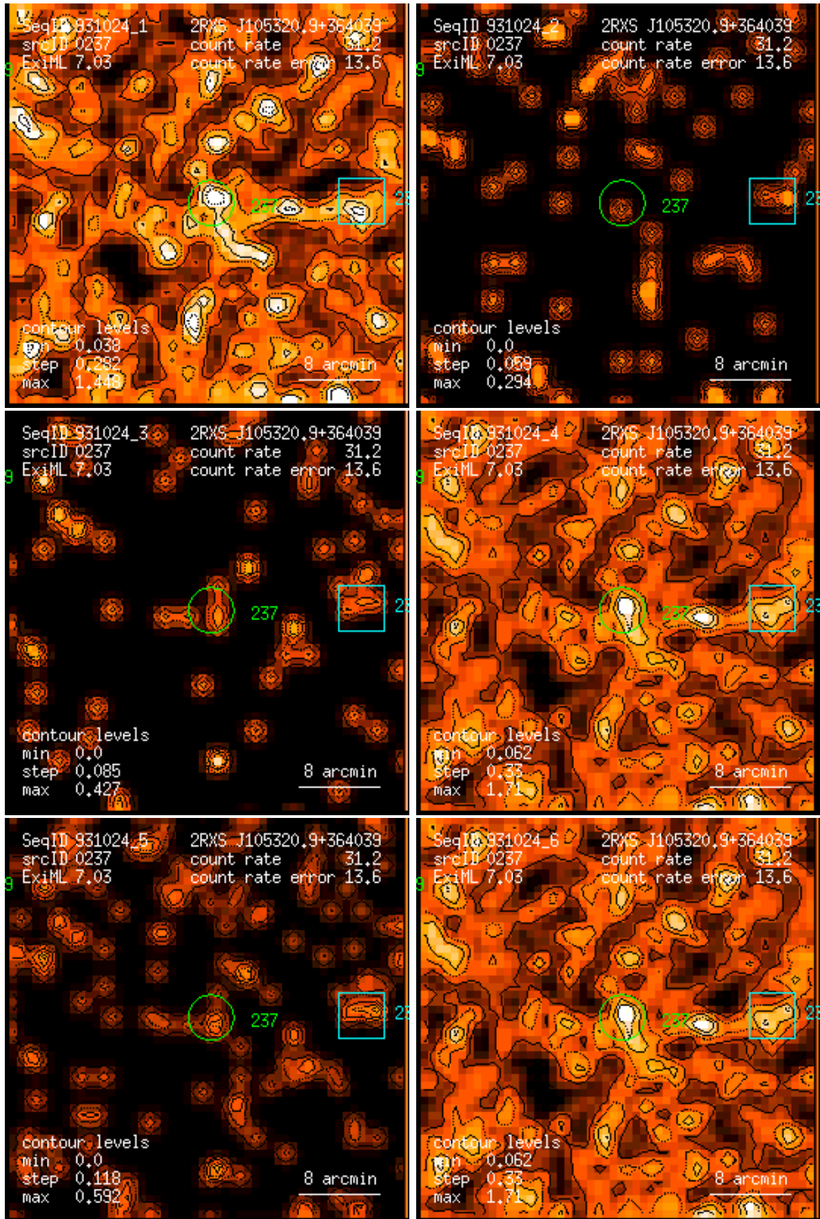
Figure 237: RASS 931024: detection 0237: band rate images, Gaussian filter: (1) PSPC channels 11 – 41, (2) 52 – 90, (3) 91 – 201, (4) 11 – 235, (5) 52 – 201, (6) 11 – 201. Broad band rates in counts/ks. Band rate contour levels in counts/ks/arcmin 2 .
