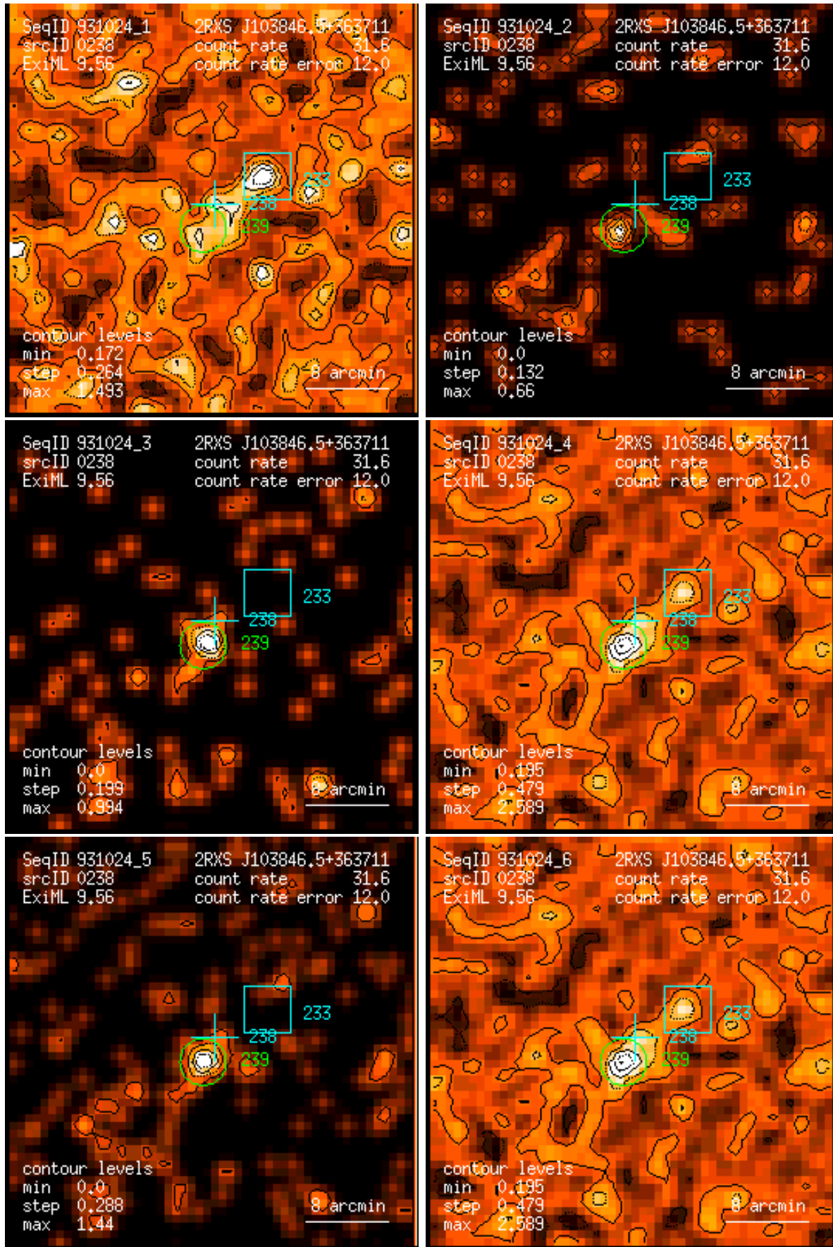
Figure 238: RASS 931024: detection 0238: band rate images, Gaussian filter: (1) PSPC channels 11 – 41, (2) 52 – 90, (3) 91 – 201, (4) 11 – 235, (5) 52 – 201, (6) 11 – 201. Broad band rates in counts/ks. Band rate contour levels in counts/ks/arcmin 2 .
