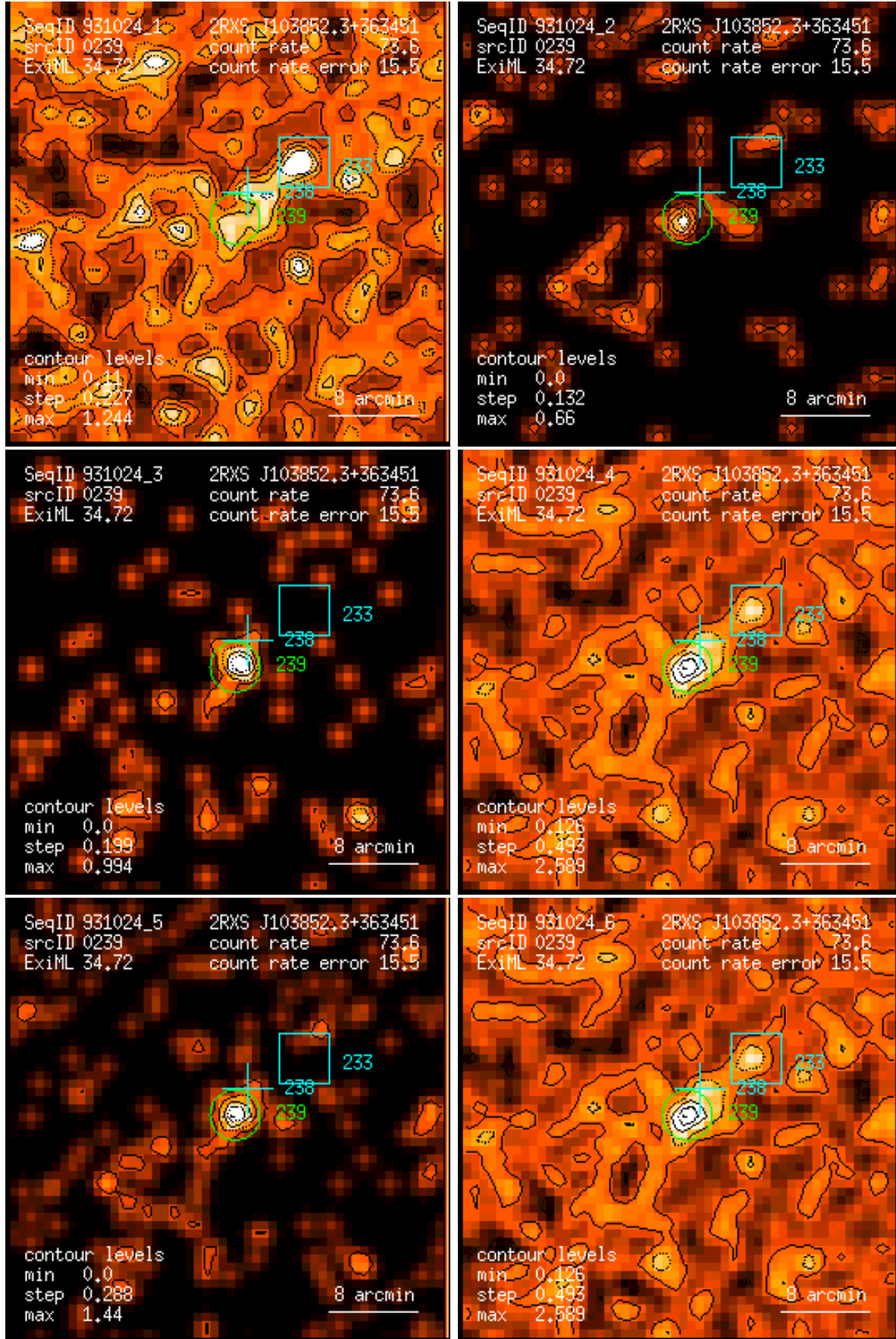
Figure 239: RASS 931024: detection 0239: band rate images, Gaussian filter: (1) PSPC channels 11 – 41, (2) 52 – 90, (3) 91 – 201, (4) 11 – 235, (5) 52 – 201, (6) 11 – 201. Broad band rates in counts/ks. Band rate contour levels in counts/ks/arcmin 2 .
