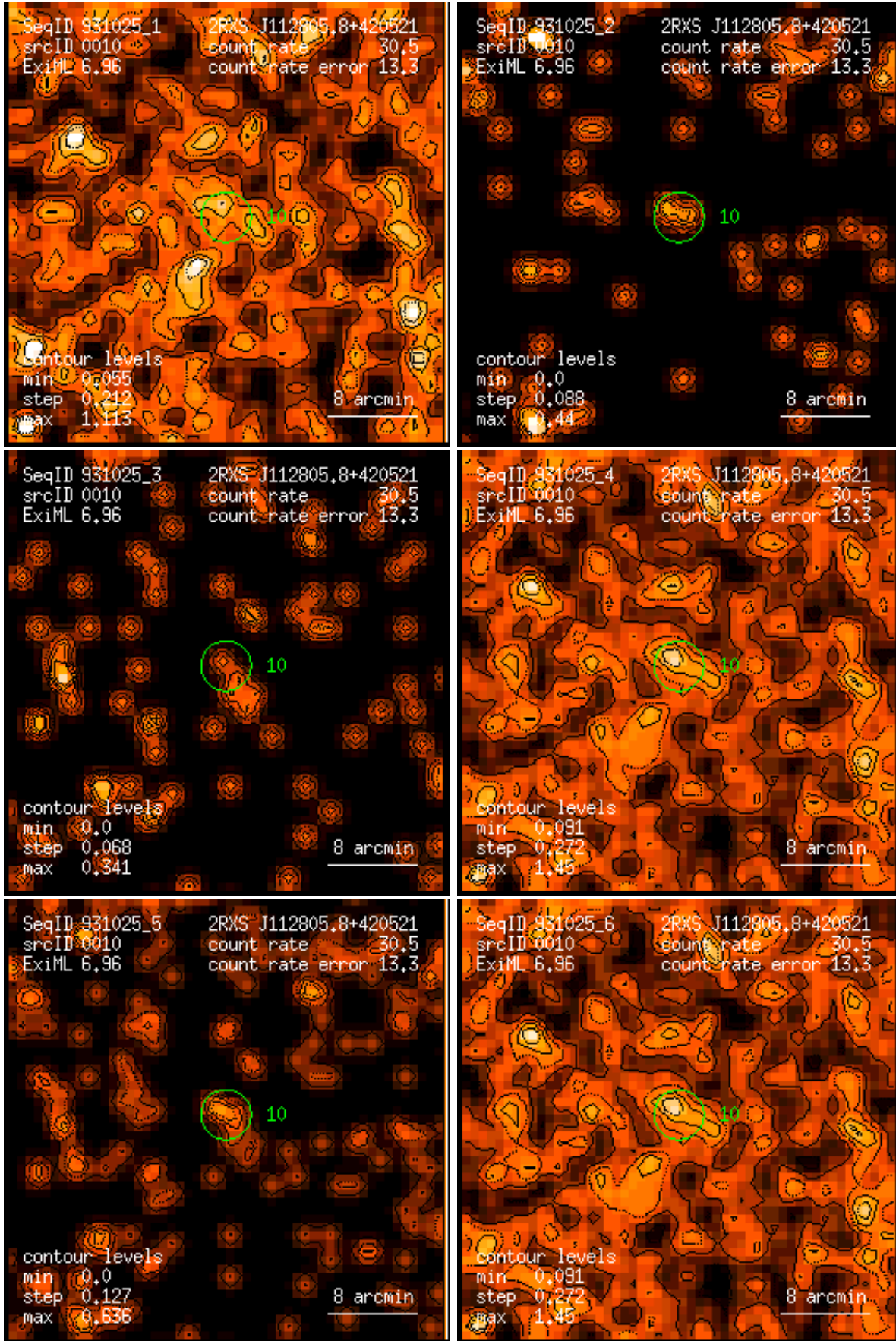
Figure 10: RASS 931025: detection 0010: band rate images, Gaussian filter: (1) PSPC channels 11 – 41, (2) 52 – 90, (3) 91 – 201, (4) 11 – 235, (5) 52 – 201, (6) 11 – 201. Broad band rates in counts/ks. Band rate contour levels in counts/ks/arcmin 2 .
