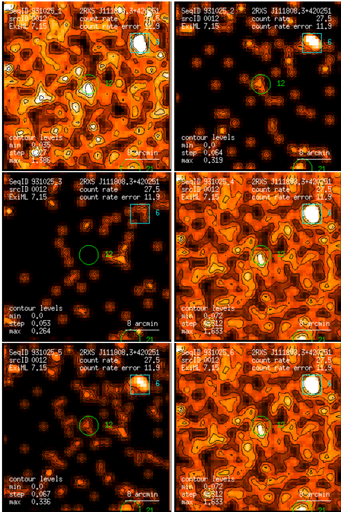
Figure 12: RASS 931025: detection 0012: band rate images, Gaussian filter: (1) PSPC channels 11 – 41, (2) 52 – 90, (3) 91 – 201, (4) 11 – 235, (5) 52 – 201, (6) 11 – 201. Broad band rates in counts/ks. Band rate contour levels in counts/ks/arcmin 2 .
