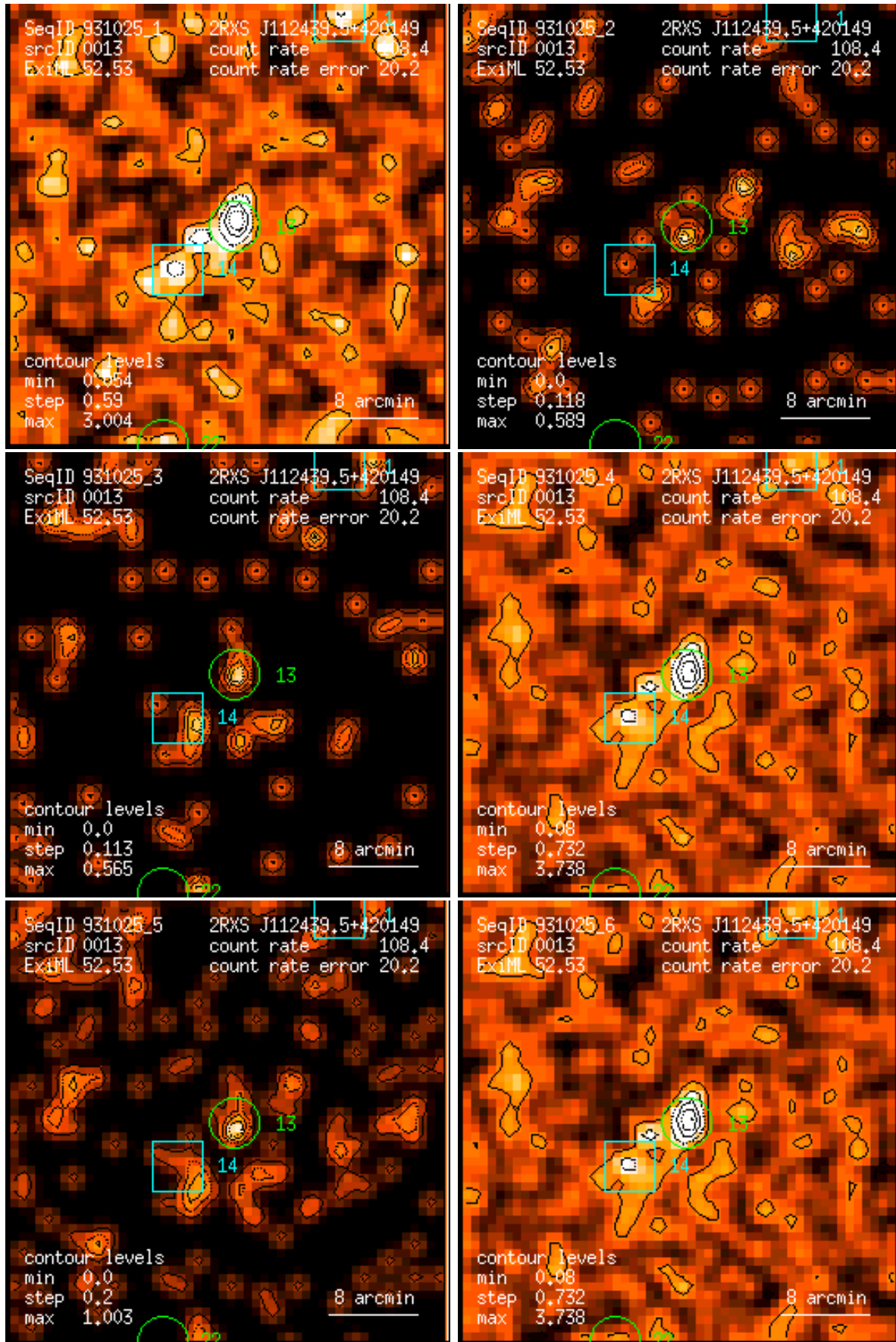
Figure 13: RASS 931025: detection 0013: band rate images, Gaussian filter: (1) PSPC channels 11 – 41, (2) 52 – 90, (3) 91 – 201, (4) 11 – 235, (5) 52 – 201, (6) 11 – 201. Broad band rates in counts/ks. Band rate contour levels in counts/ks/arcmin 2 .
