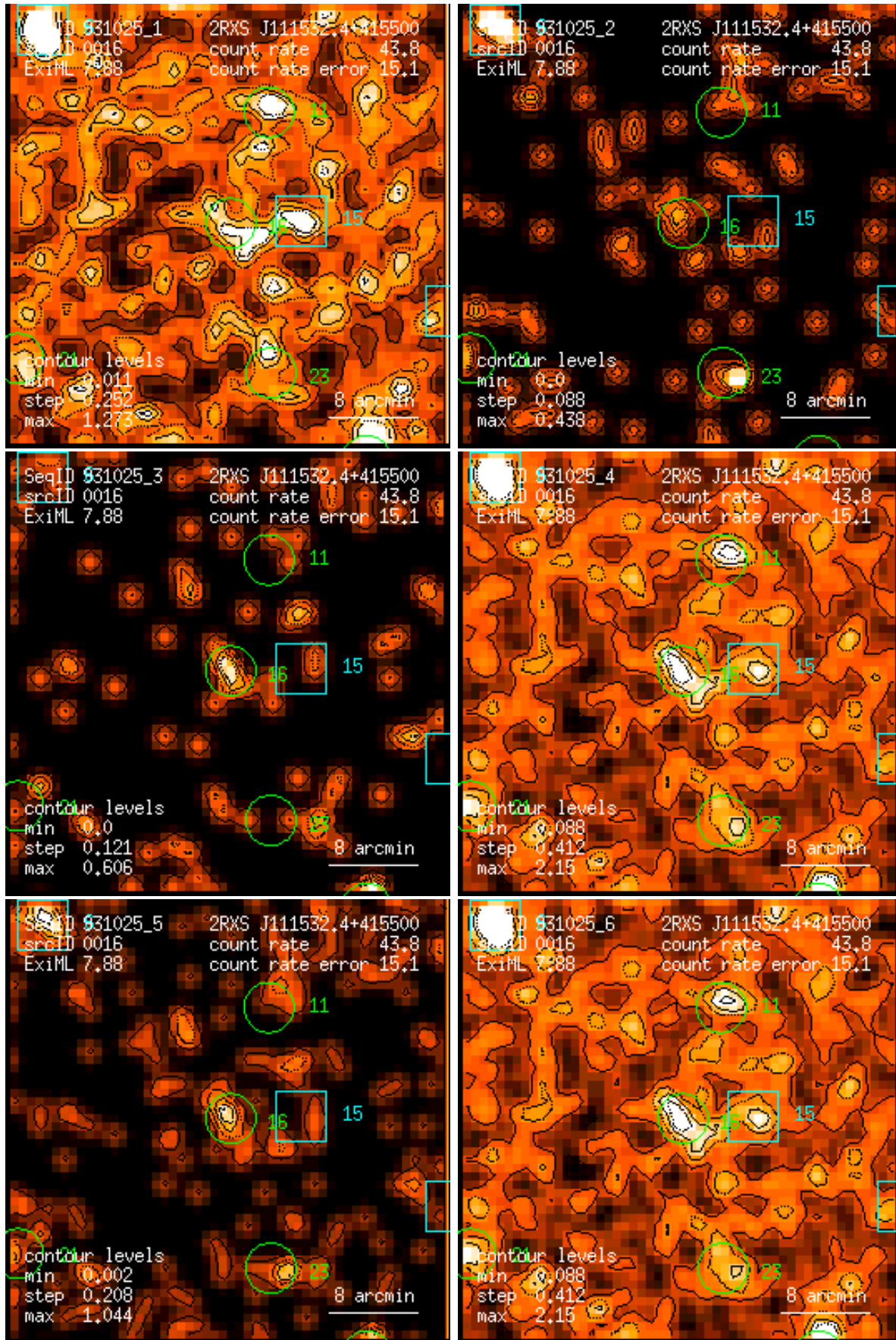
Figure 16: RASS 931025: detection 0016: band rate images, Gaussian filter: (1) PSPC channels 11 – 41, (2) 52 – 90, (3) 91 – 201, (4) 11 – 235, (5) 52 – 201, (6) 11 – 201. Broad band rates in counts/ks. Band rate contour levels in counts/ks/arcmin 2 .
