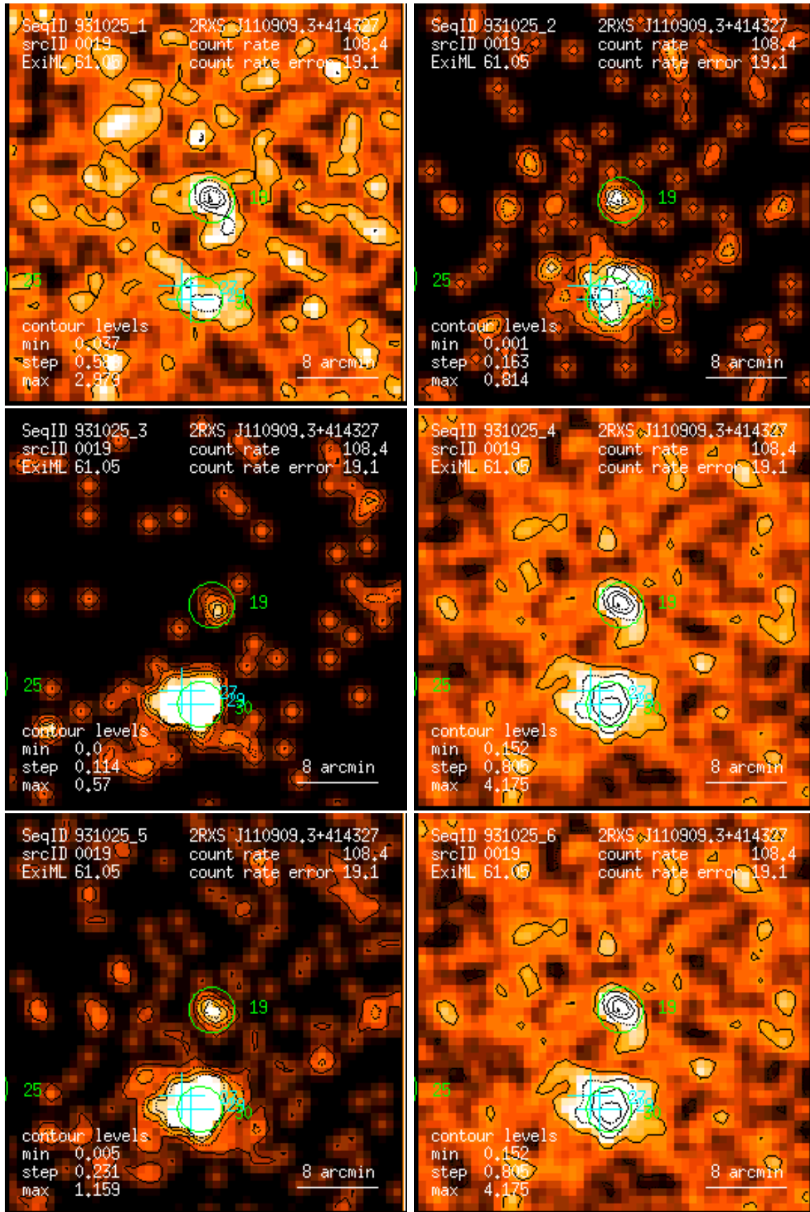
Figure 19: RASS 931025: detection 0019: band rate images, Gaussian filter: (1) PSPC channels 11 – 41, (2) 52 – 90, (3) 91 – 201, (4) 11 – 235, (5) 52 – 201, (6) 11 – 201. Broad band rates in counts/ks. Band rate contour levels in counts/ks/arcmin 2 .
