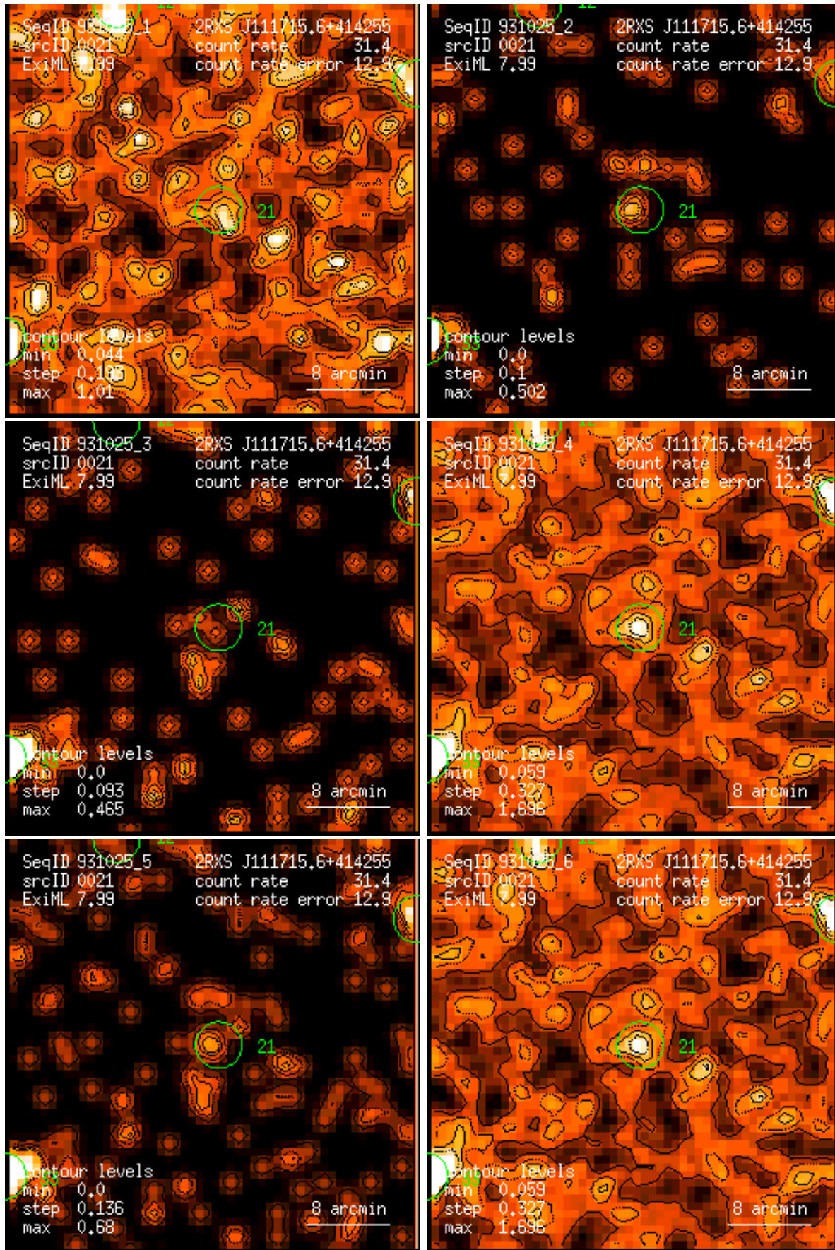
Figure 21: RASS 931025: detection 0021: band rate images, Gaussian filter: (1) PSPC channels 11 – 41, (2) 52 – 90, (3) 91 – 201, (4) 11 – 235, (5) 52 – 201, (6) 11 – 201. Broad band rates in counts/ks. Band rate contour levels in counts/ks/arcmin 2 .
