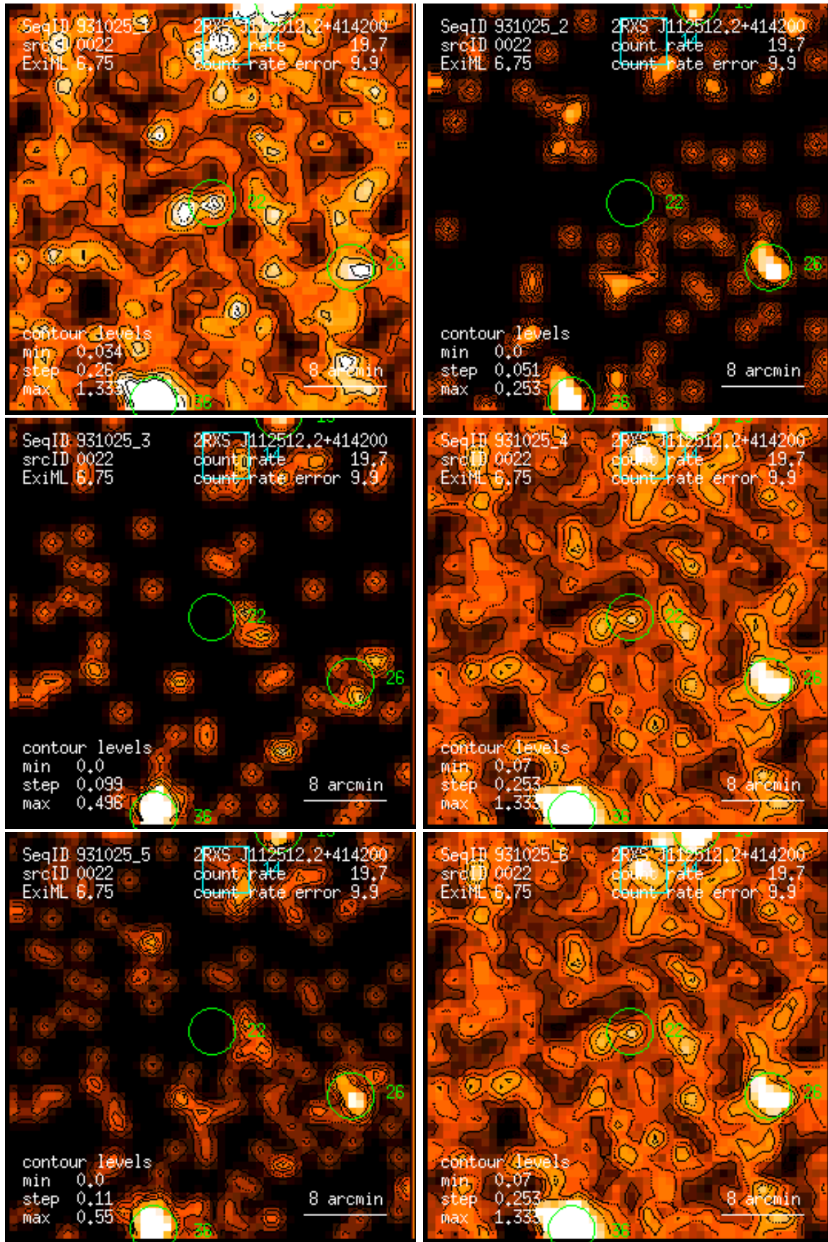
Figure 22: RASS 931025: detection 0022: band rate images, Gaussian filter: (1) PSPC channels 11 – 41, (2) 52 – 90, (3) 91 – 201, (4) 11 – 235, (5) 52 – 201, (6) 11 – 201. Broad band rates in counts/ks. Band rate contour levels in counts/ks/arcmin 2 .
