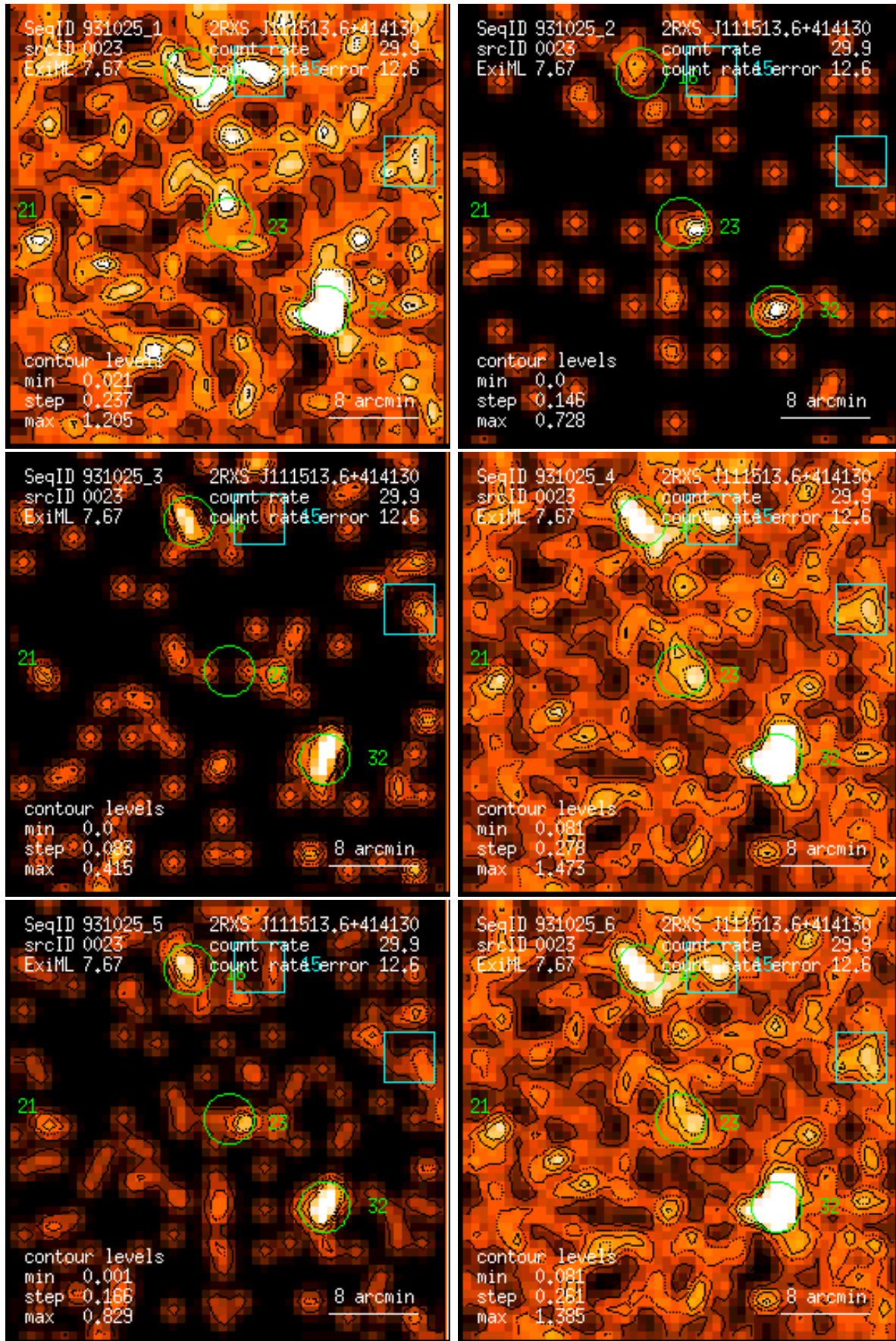
Figure 23: RASS 931025: detection 0023: band rate images, Gaussian filter: (1) PSPC channels 11 – 41, (2) 52 – 90, (3) 91 – 201, (4) 11 – 235, (5) 52 – 201, (6) 11 – 201. Broad band rates in counts/ks. Band rate contour levels in counts/ks/arcmin 2 .
