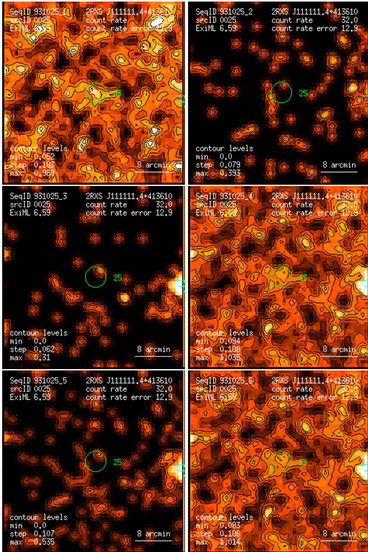
Figure 25: RASS 931025: detection 0025: band rate images, Gaussian filter: (1) PSPC channels 11 – 41, (2) 52 – 90, (3) 91 – 201, (4) 11 – 235, (5) 52 – 201, (6) 11 – 201. Broad band rates in counts/ks. Band rate contour levels in counts/ks/arcmin 2 .
