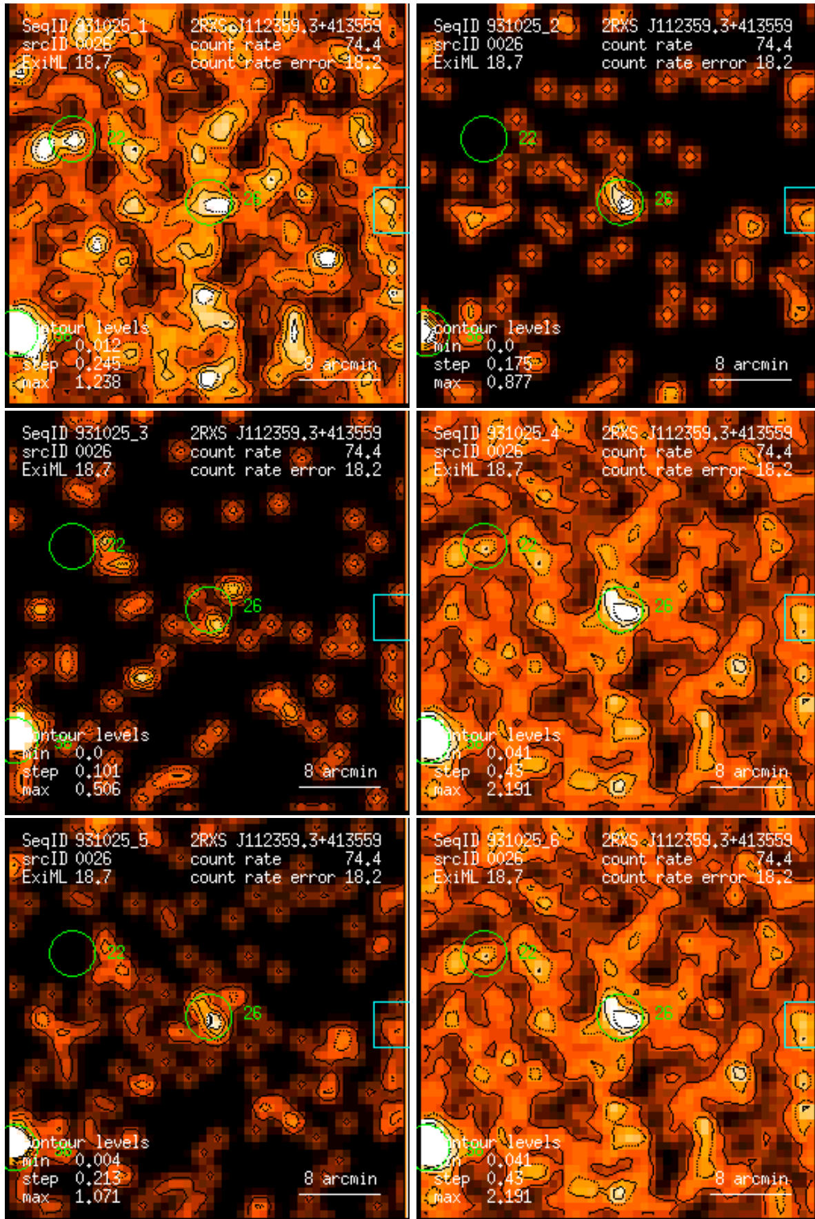
Figure 26: RASS 931025: detection 0026: band rate images, Gaussian filter: (1) PSPC channels 11 – 41, (2) 52 – 90, (3) 91 – 201, (4) 11 – 235, (5) 52 – 201, (6) 11 – 201. Broad band rates in counts/ks. Band rate contour levels in counts/ks/arcmin 2 .
