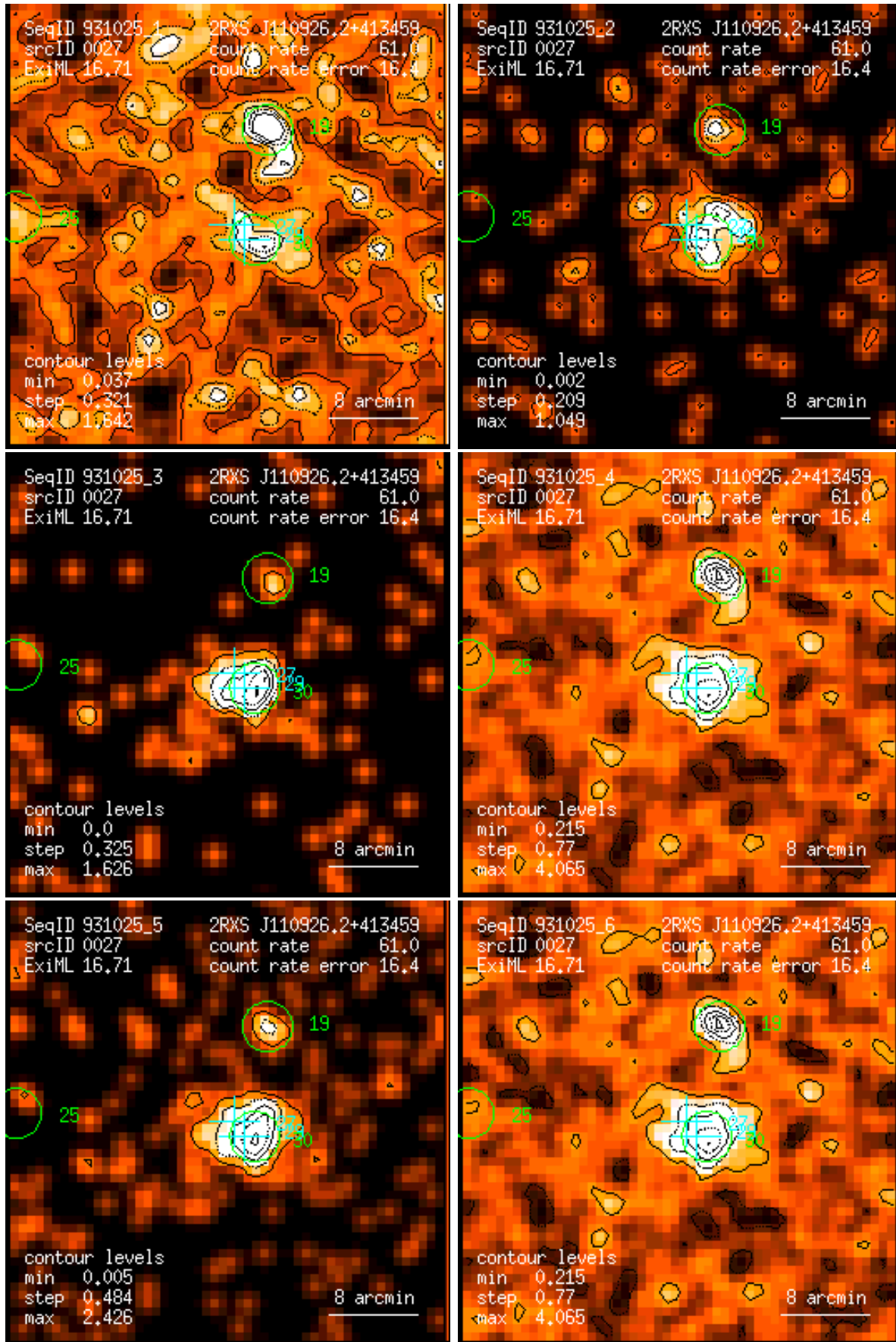
Figure 27: RASS 931025: detection 0027: band rate images, Gaussian filter: (1) PSPC channels 11 – 41, (2) 52 – 90, (3) 91 – 201, (4) 11 – 235, (5) 52 – 201, (6) 11 – 201. Broad band rates in counts/ks. Band rate contour levels in counts/ks/arcmin 2 .
