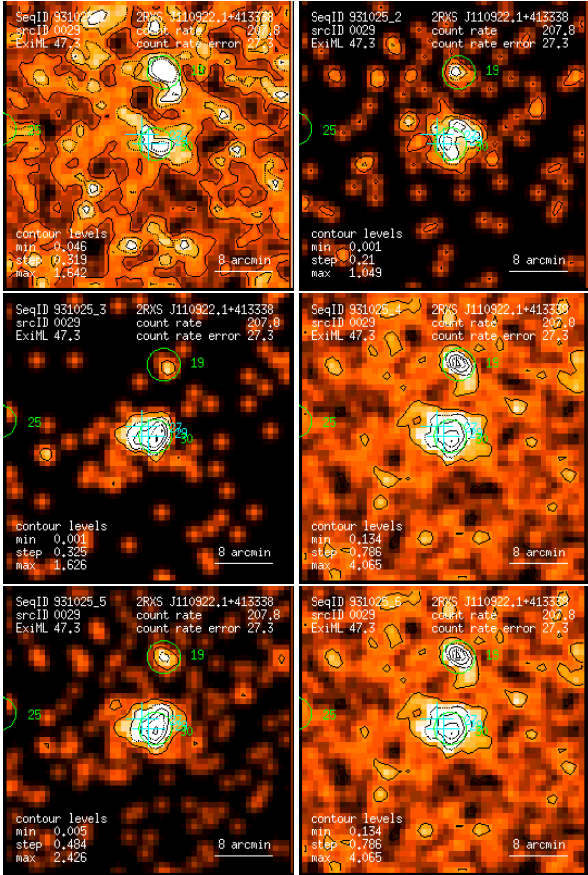
Figure 29: RASS 931025: detection 0029: band rate images, Gaussian filter: (1) PSPC channels 11 – 41, (2) 52 – 90, (3) 91 – 201, (4) 11 – 235, (5) 52 – 201, (6) 11 – 201. Broad band rates in counts/ks. Band rate contour levels in counts/ks/arcmin 2 .
