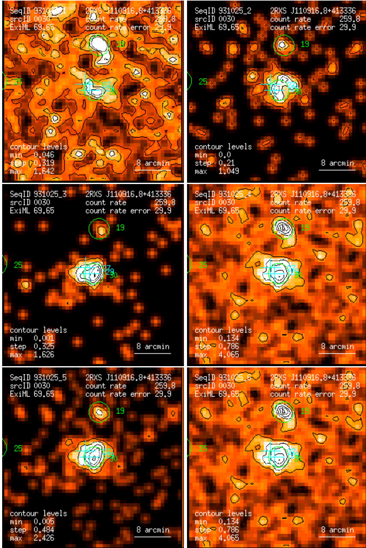
Figure 30: RASS 931025: detection 0030: band rate images, Gaussian filter: (1) PSPC channels 11 – 41, (2) 52 – 90, (3) 91 – 201, (4) 11 – 235, (5) 52 – 201, (6) 11 – 201. Broad band rates in counts/ks. Band rate contour levels in counts/ks/arcmin 2 .
