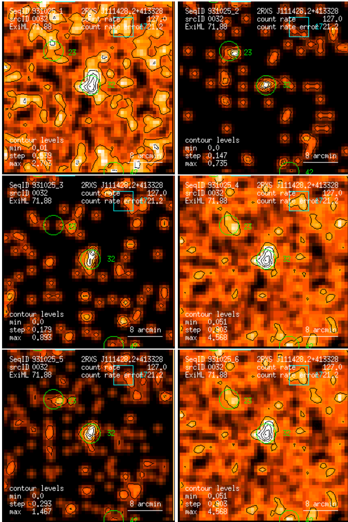
Figure 32: RASS 931025: detection 0032: band rate images, Gaussian filter: (1) PSPC channels 11 – 41, (2) 52 – 90, (3) 91 – 201, (4) 11 – 235, (5) 52 – 201, (6) 11 – 201. Broad band rates in counts/ks. Band rate contour levels in counts/ks/arcmin 2 .
