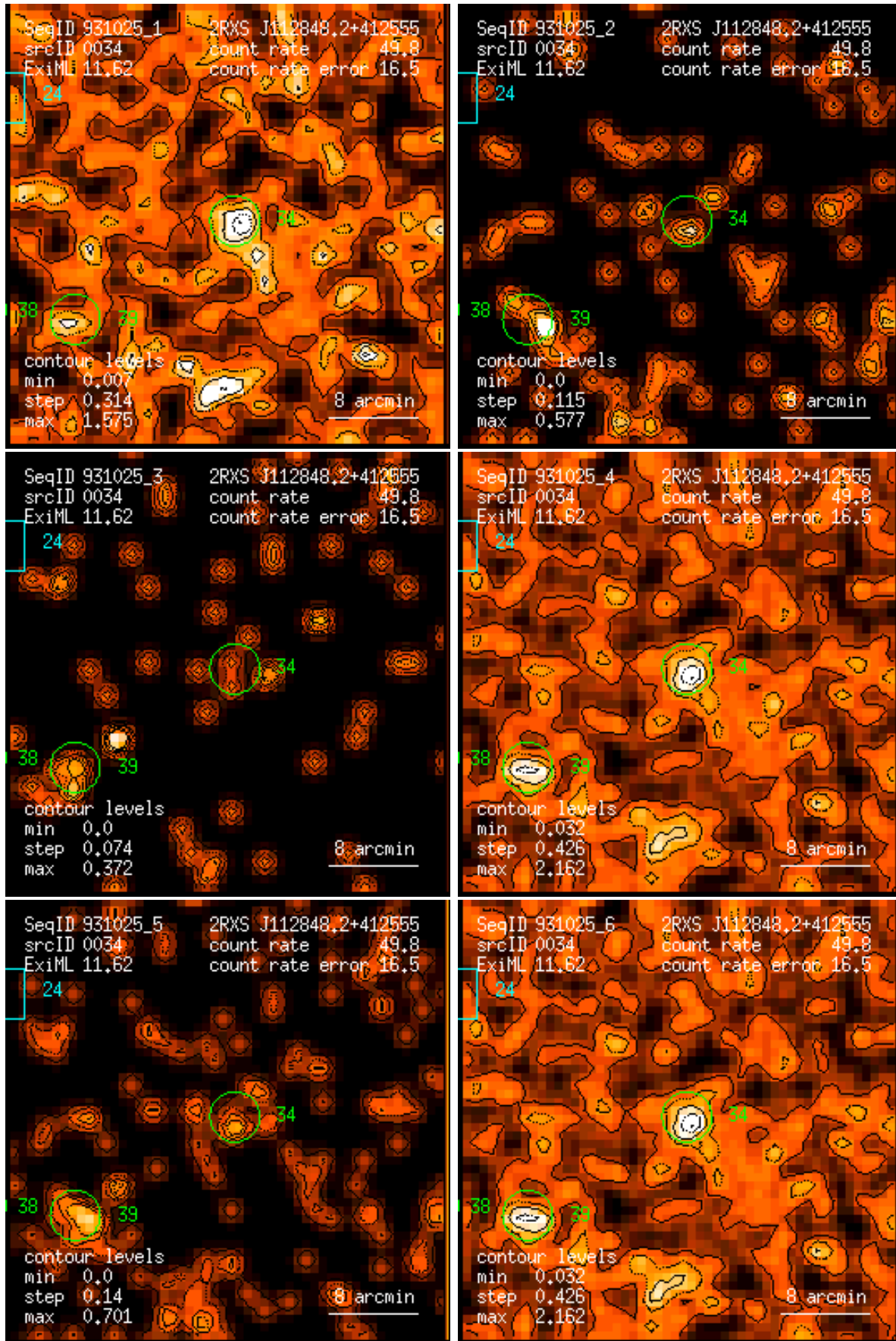
Figure 34: RASS 931025: detection 0034: band rate images, Gaussian filter: (1) PSPC channels 11 – 41, (2) 52 – 90, (3) 91 – 201, (4) 11 – 235, (5) 52 – 201, (6) 11 – 201. Broad band rates in counts/ks. Band rate contour levels in counts/ks/arcmin 2 .
