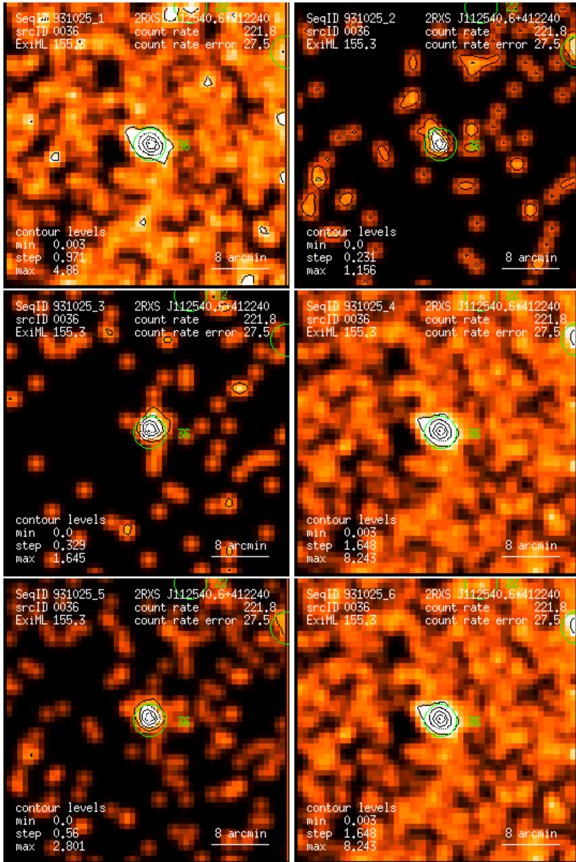
Figure 36: RASS 931025: detection 0036: band rate images, Gaussian filter: (1) PSPC channels 11 – 41, (2) 52 – 90, (3) 91 – 201, (4) 11 – 235, (5) 52 – 201, (6) 11 – 201. Broad band rates in counts/ks. Band rate contour levels in counts/ks/arcmin 2 .
