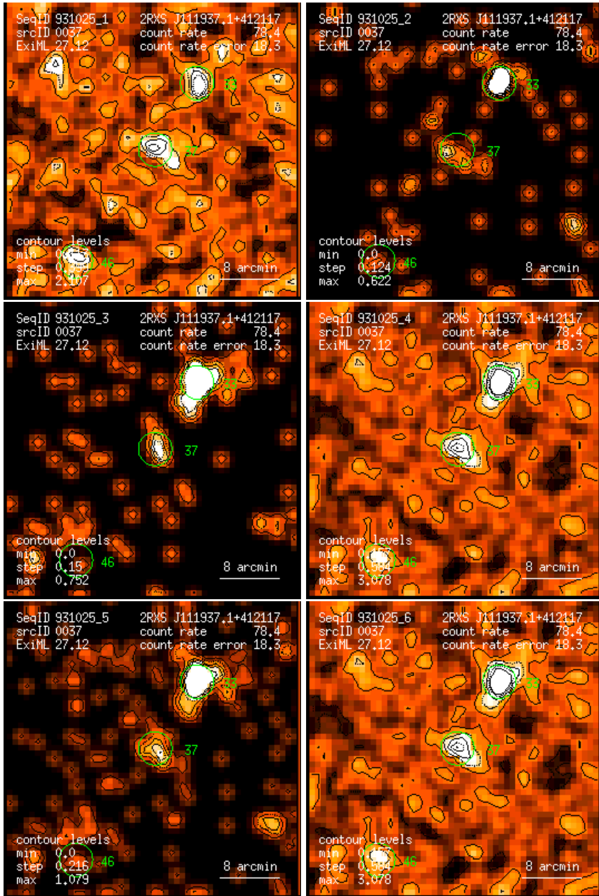
Figure 37: RASS 931025: detection 0037: band rate images, Gaussian filter: (1) PSPC channels 11 – 41, (2) 52 – 90, (3) 91 – 201, (4) 11 – 235, (5) 52 – 201, (6) 11 – 201. Broad band rates in counts/ks. Band rate contour levels in counts/ks/arcmin 2 .
