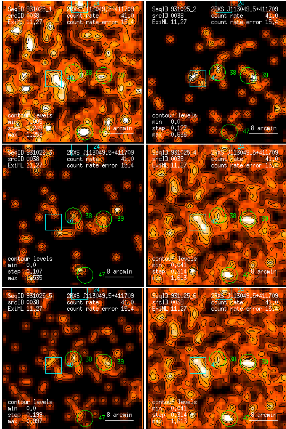
Figure 38: RASS 931025: detection 0038: band rate images, Gaussian filter: (1) PSPC channels 11 – 41, (2) 52 – 90, (3) 91 – 201, (4) 11 – 235, (5) 52 – 201, (6) 11 – 201. Broad band rates in counts/ks. Band rate contour levels in counts/ks/arcmin 2 .
