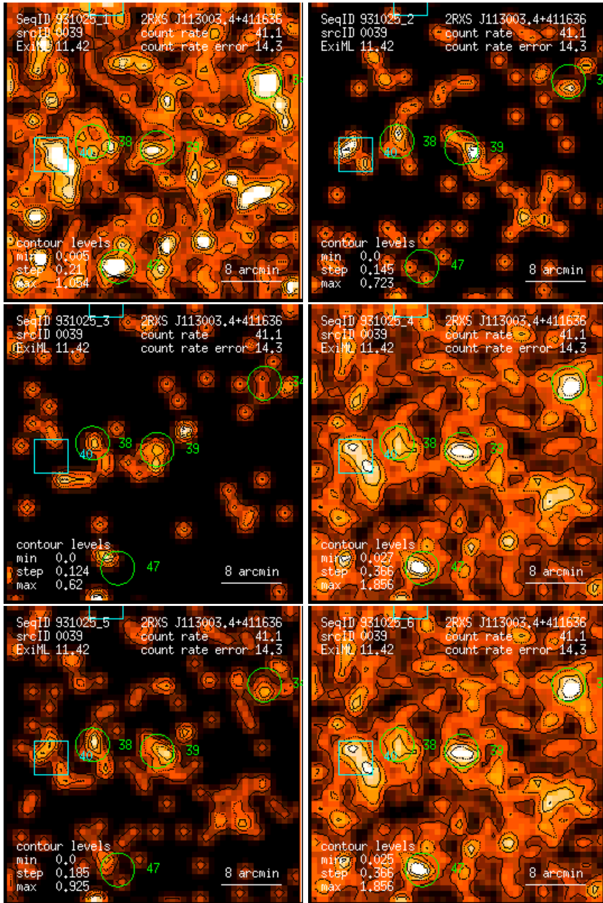
Figure 39: RASS 931025: detection 0039: band rate images, Gaussian filter: (1) PSPC channels 11 – 41, (2) 52 – 90, (3) 91 – 201, (4) 11 – 235, (5) 52 – 201, (6) 11 – 201. Broad band rates in counts/ks. Band rate contour levels in counts/ks/arcmin 2 .
